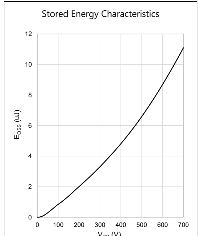
Figure 8: Typical C_{OSS} Stored Energy
