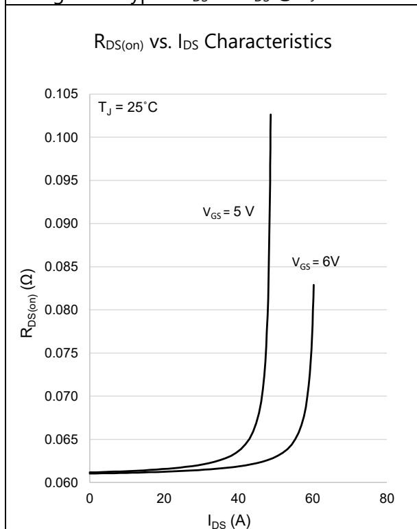
Figure 3: R_{DS(on)} vs. I_{DS} at T_J = 25^\circ\text{C}
