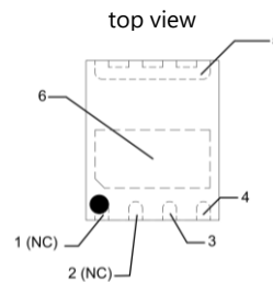
Package Outline
