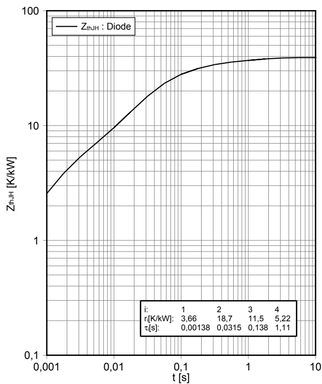
瞬态热阻抗 二极管,逆变器 transient thermal impedance Diode, Inverter Z_{thJH} = f(t)
