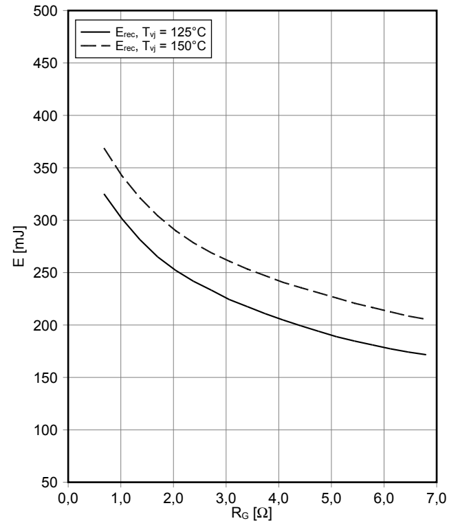
开关损耗 二极管,逆变器 (典型) switching losses Diode, Inverter (typical) E_{rec} = f(R_G) I_F = 1200 A , V_{CE} = 900 V
