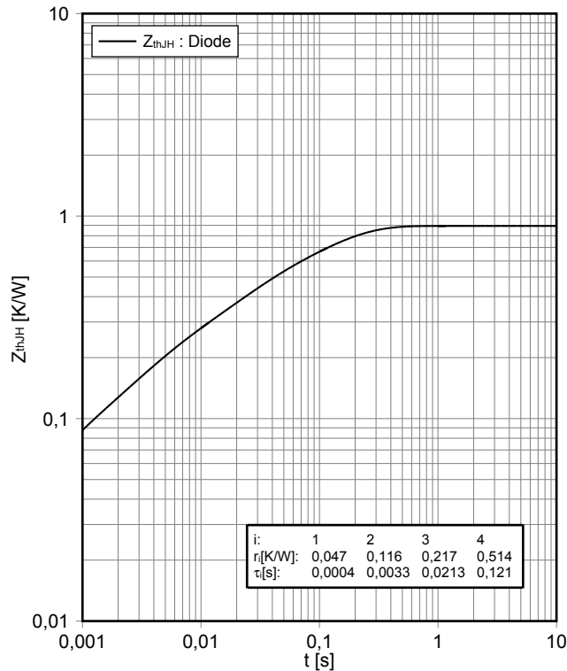
Transienter Wärmewiderstand Bypass-Diode transient thermal impedance Bypass-Diode Z_{thJH} = f(t)
