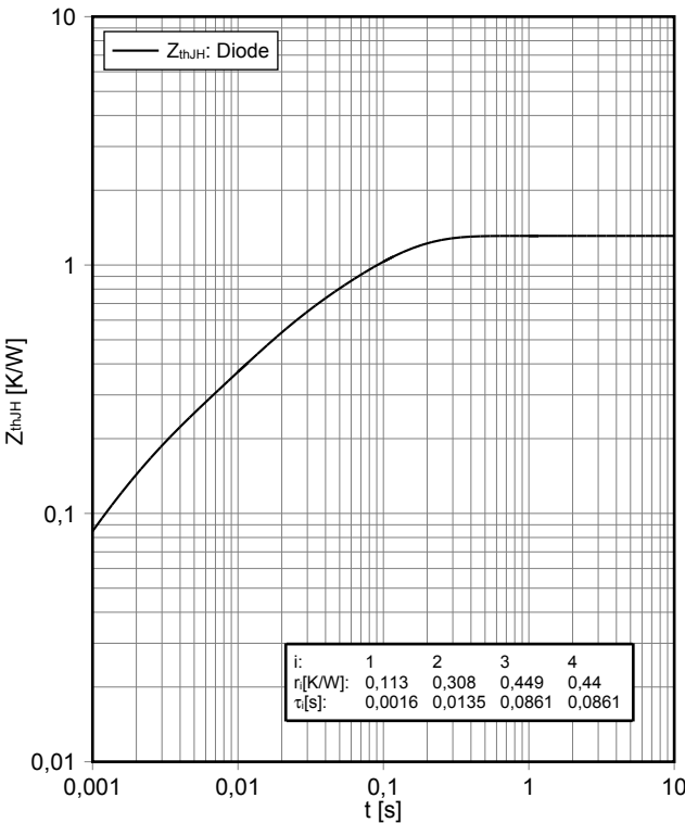
Transienter Wärmewiderstand Verpolschutz Diode A transient thermal impedance Inverse-polarity protection diode A Z_{thJH} = f(t)
