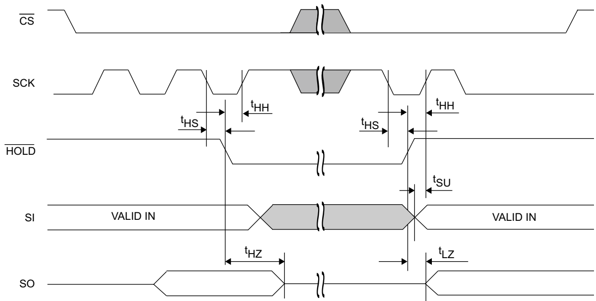
Figure 14. \overline{HOLD} Timing
