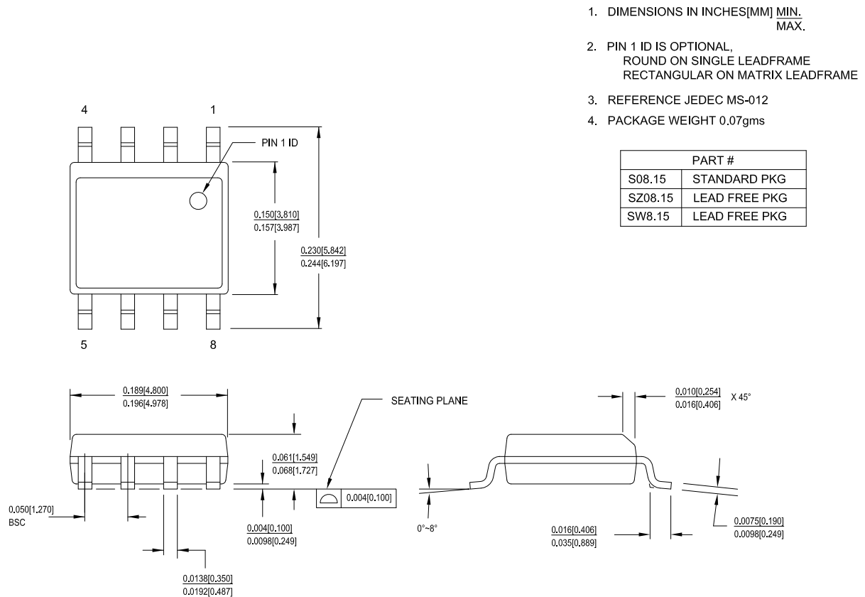
Figure 22. 8-pin SOIC (150 Mils) Package Outline, 51-85066
