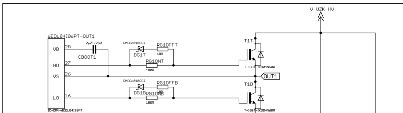
Figure 4 Gate driver output of the 6EDL04I06PT. Exemplarily only 1 phase output pictured
