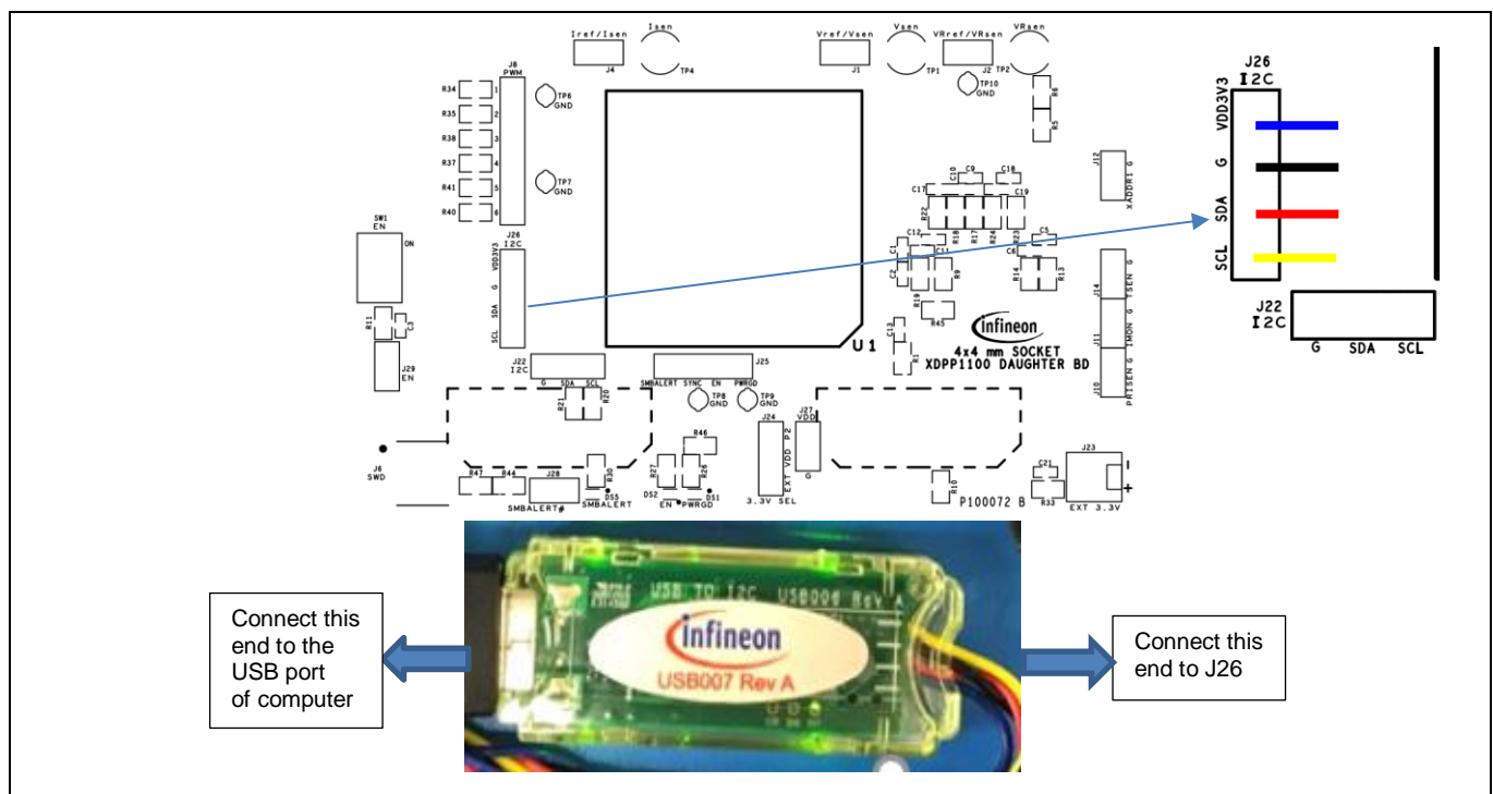
Figure 6 USB-to-I²C dongle connection
