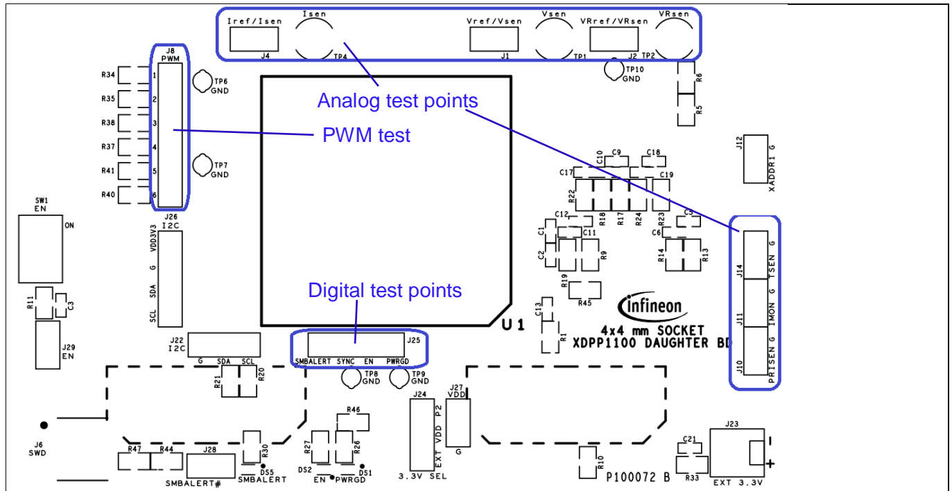
Figure 3 XDPP1100-Q024 test points
