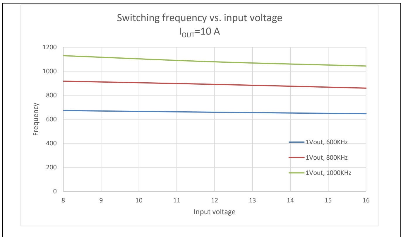
Figure 19 Switching frequency vs. input voltage
