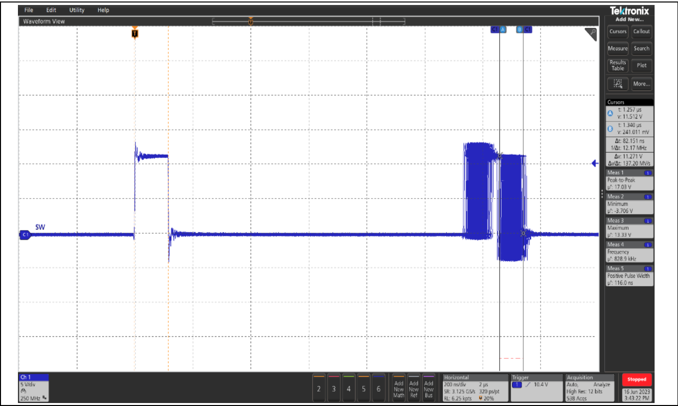
Figure 14 SW node, 12 A load, F_{sw} = 800 kHz
