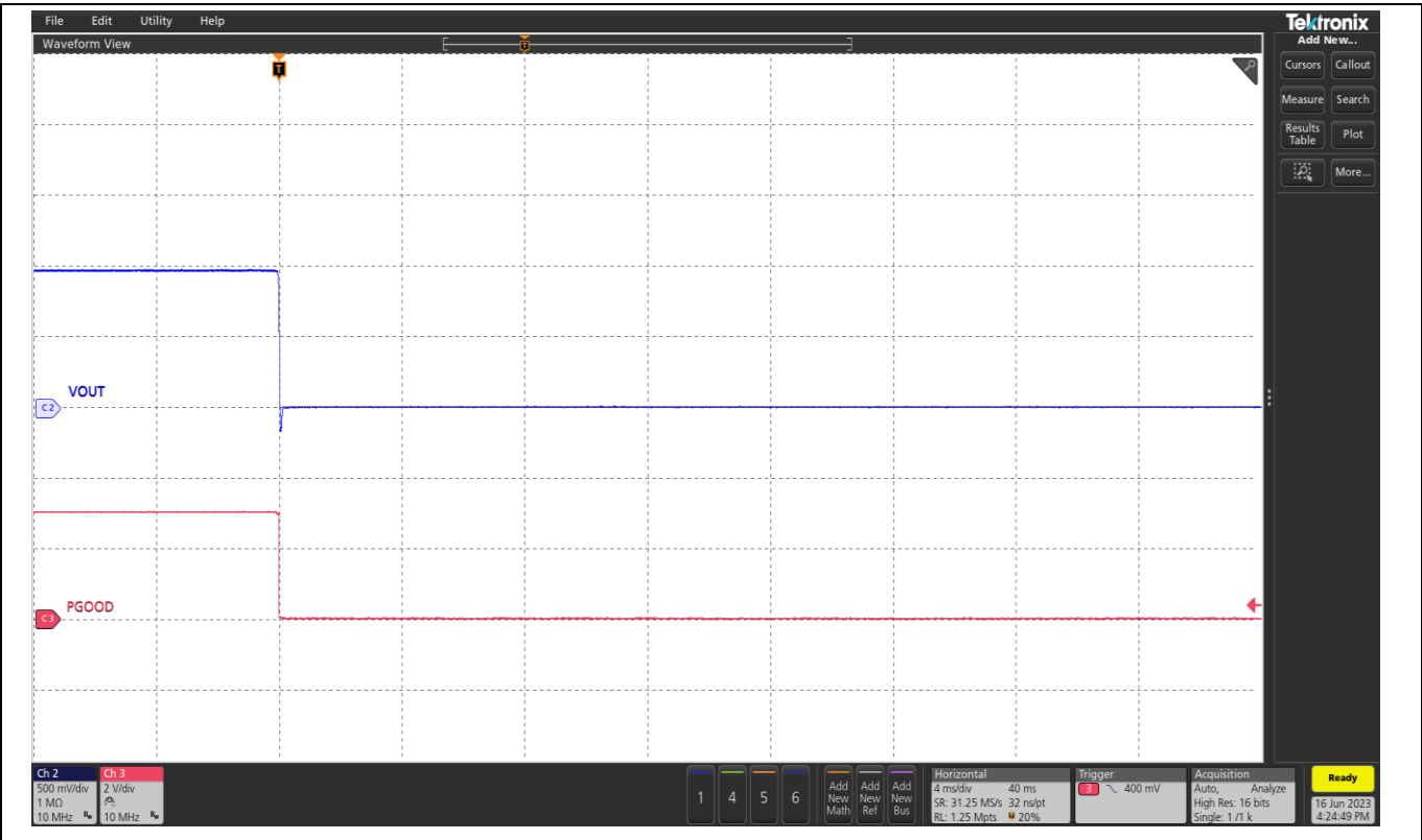
Figure 16 Short circuit and UVP (shutdown), (Ch2: V OUT , Ch3:P GOOD )
