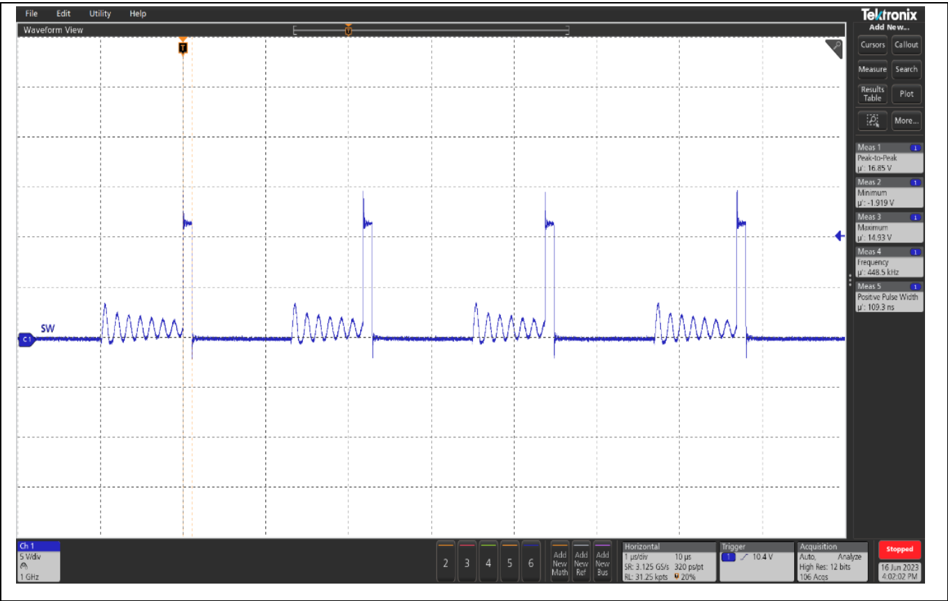
Figure 15 SW node (in DEM), 1 A load
