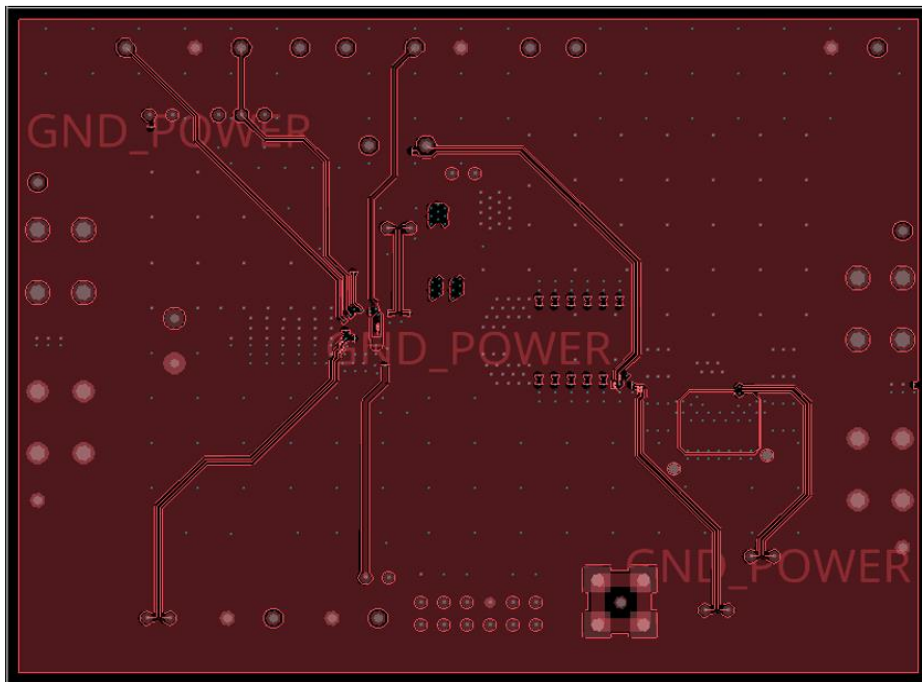
Figure 5 Inner layer 2
