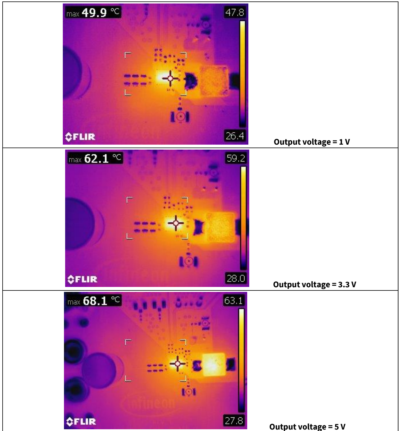
Figure 20 Thermal performance of TDA38813 for 1 V, 3.3 V, and 5 V output voltages, 12 A load, FCCM mode, 800 kHz switching frequency, 12 V V_{IN}
