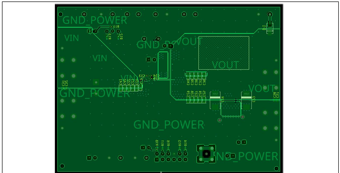
Figure 3 Bottom layer
