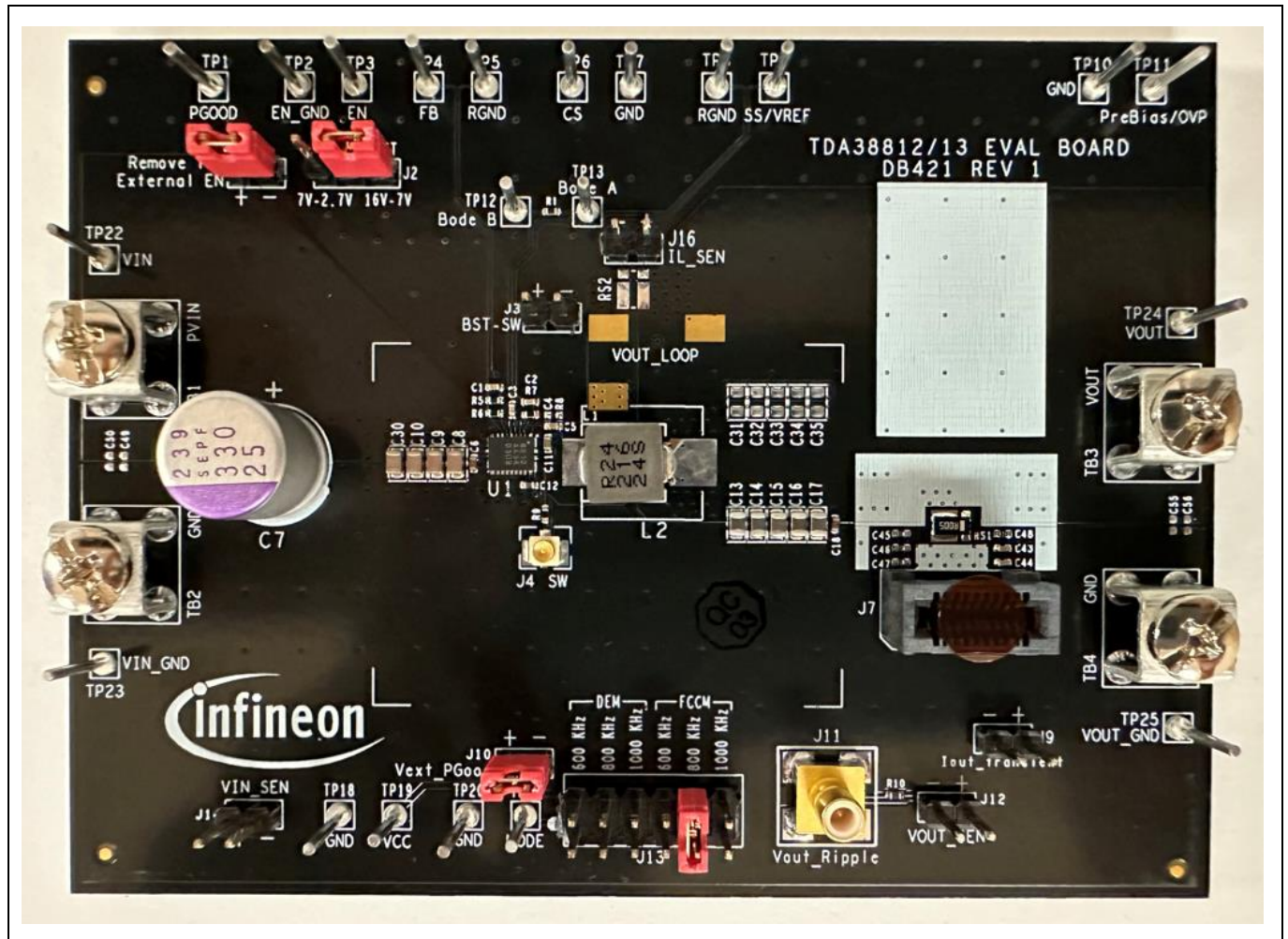
Figure 1 Evaluation board
