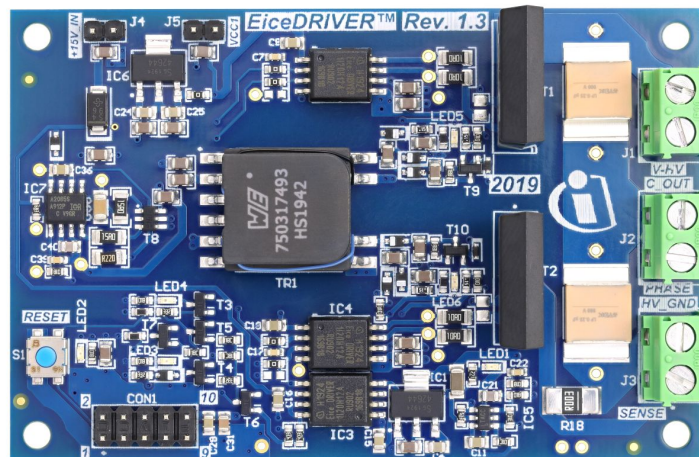
Figure 1 EVAL-1EDC20H12AH-SIC top view
