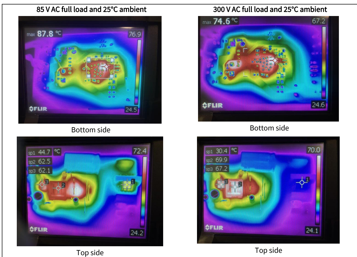
Figure 17 Infrared thermal image of DEMO_5GR4780AG_14W1
