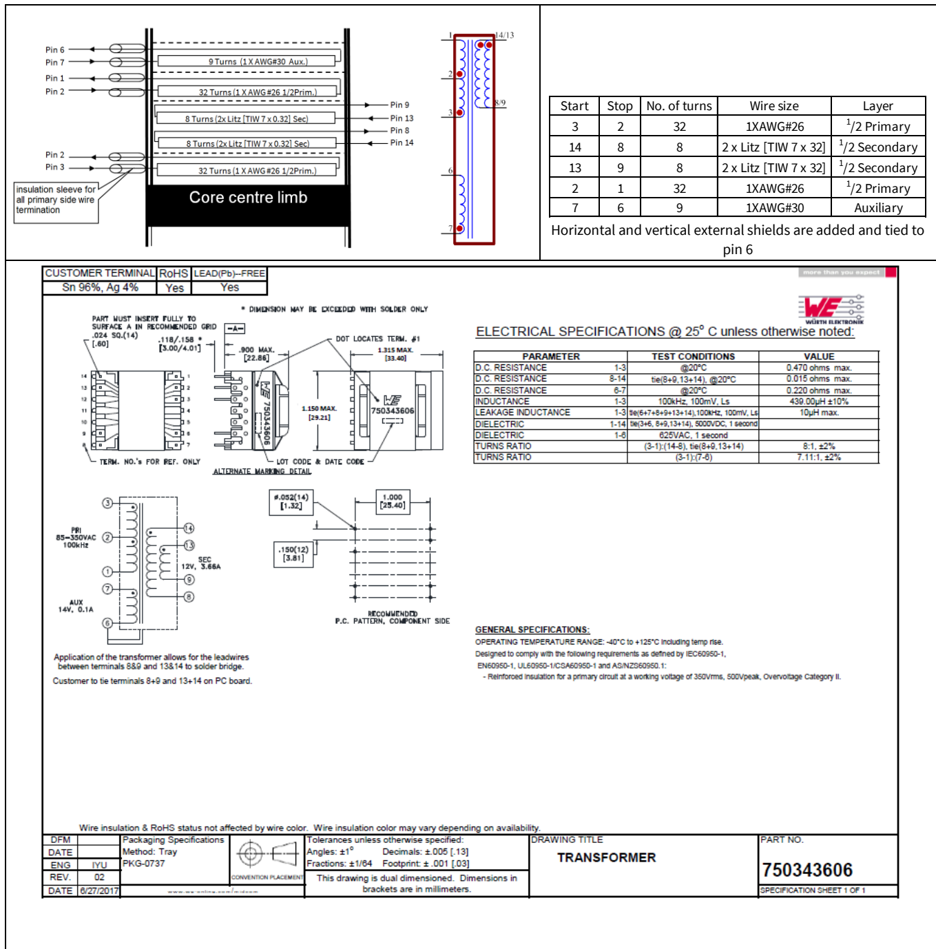
Figure 7 Transformer structure
