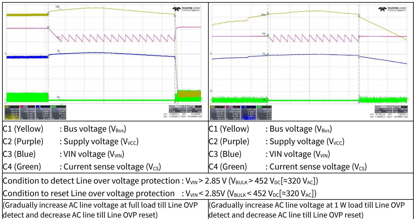
Figure 30 Line over voltage protection at 320 V_{AC}
