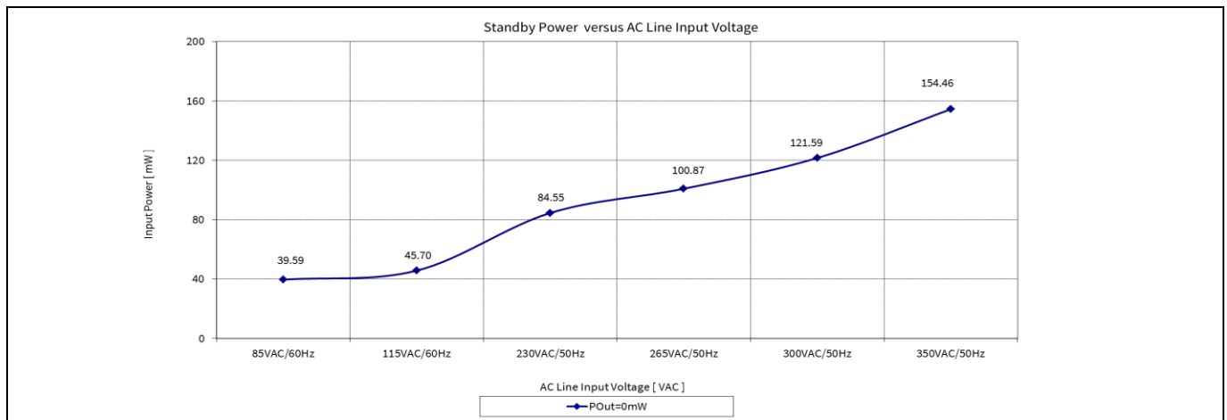
Figure 11 Standby power at no-load vs AC-line input voltage (measured by Yokogawa WT210 power meter – integration mode)
