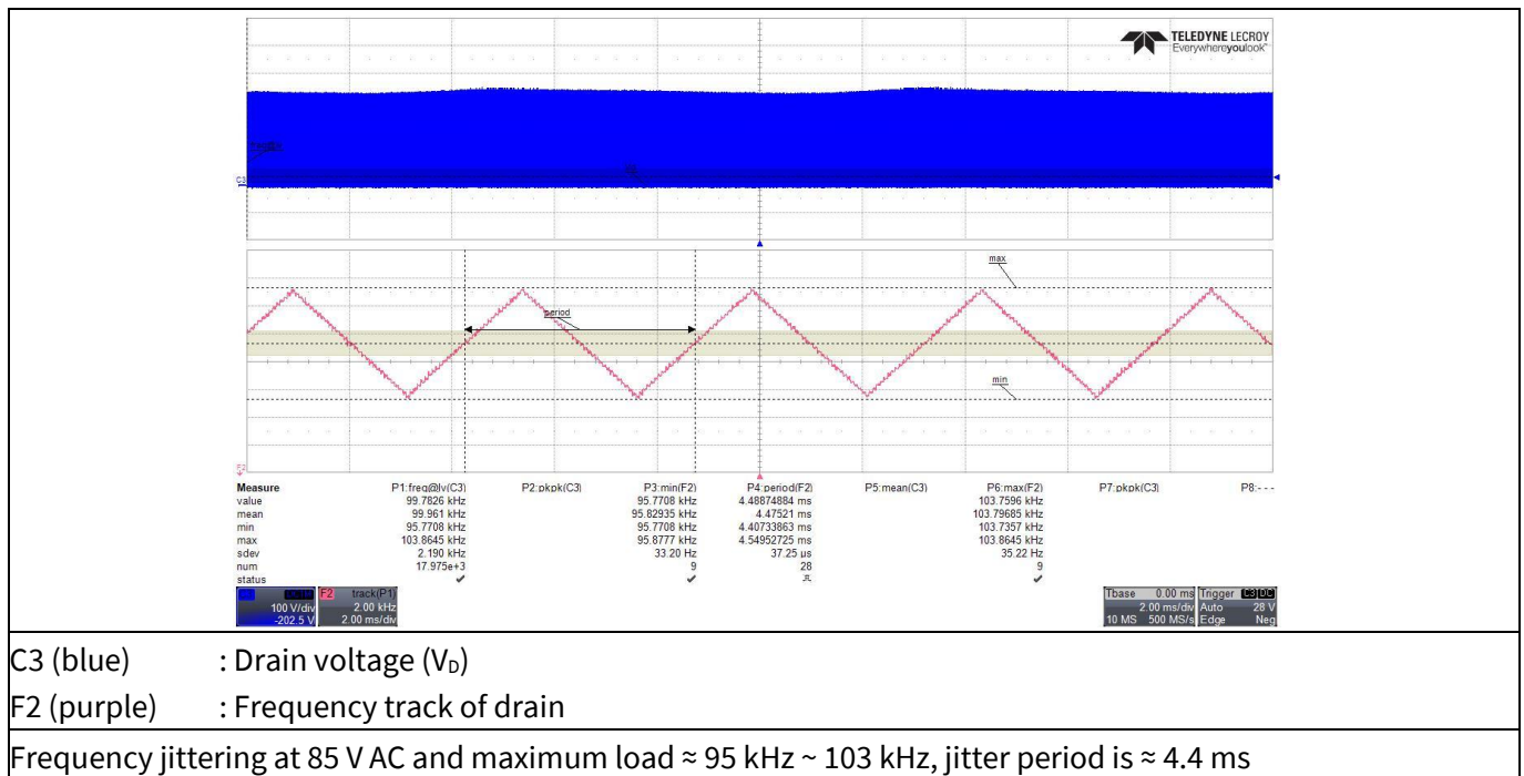
Figure 23 Frequency jittering
