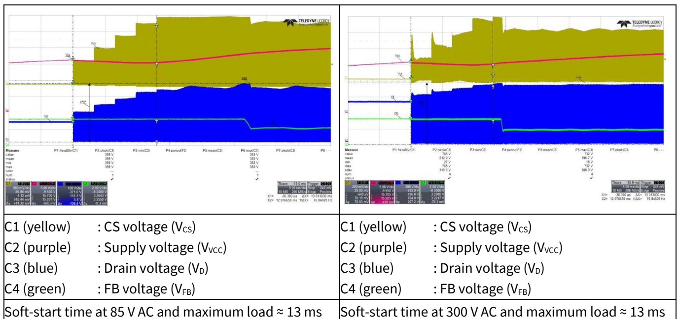
Figure 21 Soft-start
