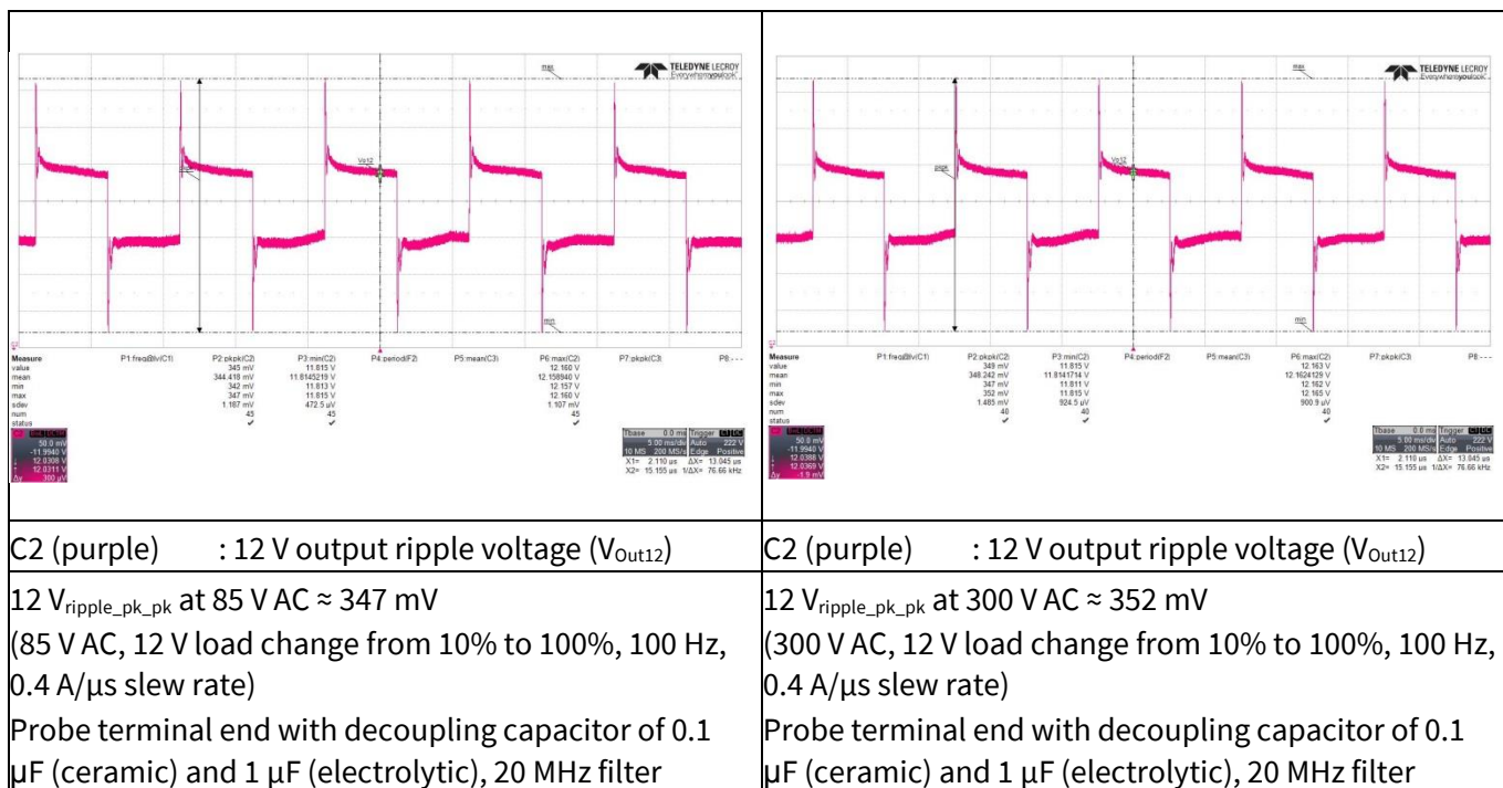
Figure 24 Load transient response
