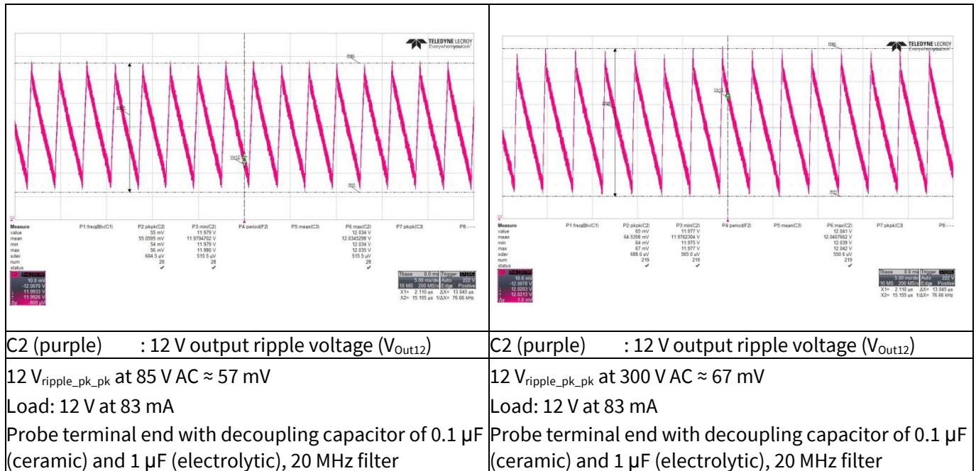
Figure 26 Output ripple voltage at burst mode 1 W load
