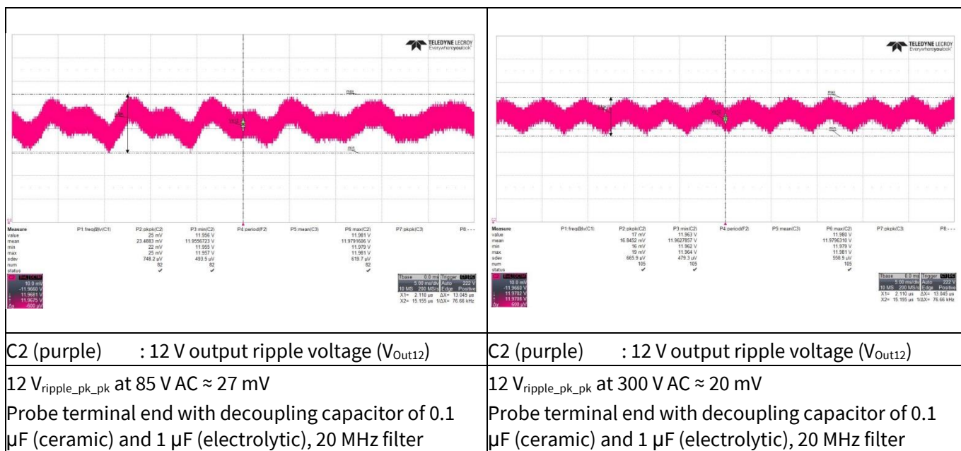
Figure 25 Output ripple voltage at maximum load
