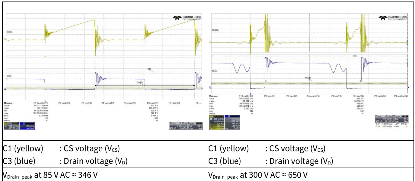
Figure 22 Drain and CS voltage at maximum load
