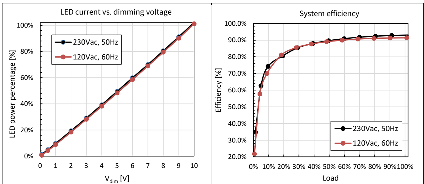
Figure 10 LED current vs. dimming voltage ( V_{LED} = 76 V)
