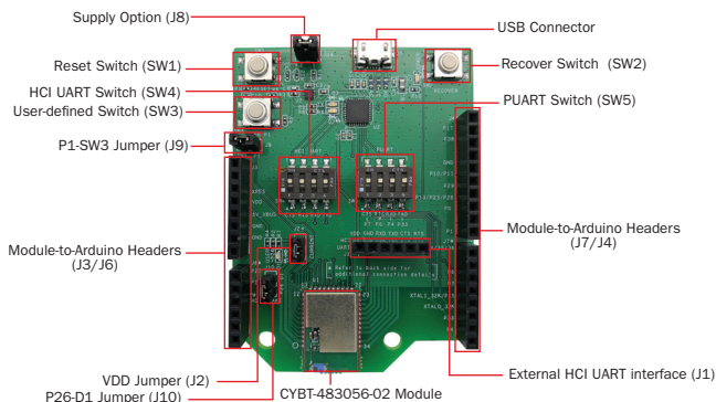
Figure 1: CYBT-483056-EVAL Top View
