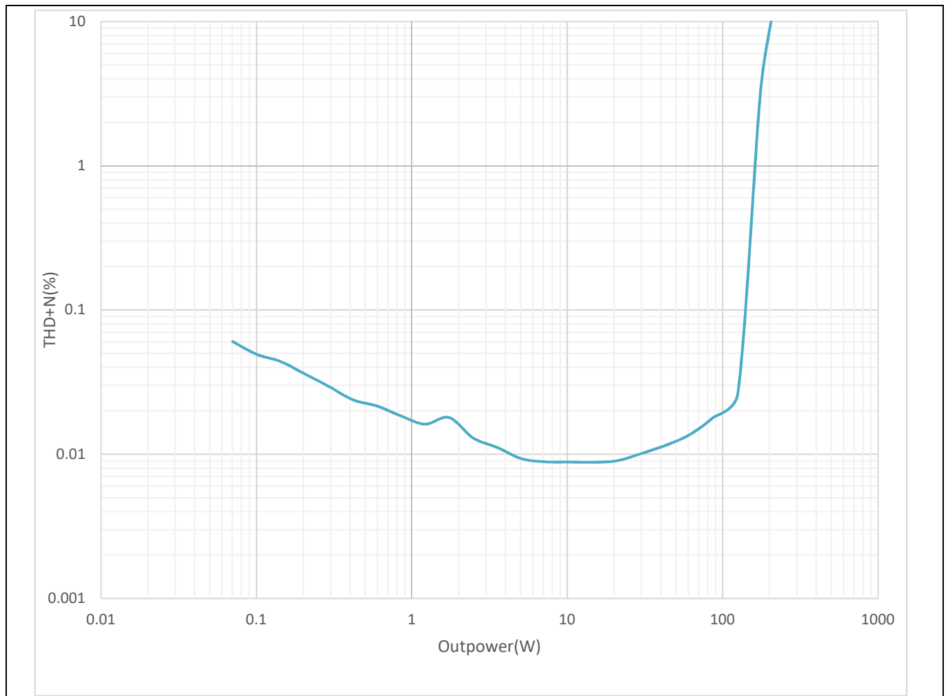
Figure 4 Power vs. THD+N 8 Ω load
