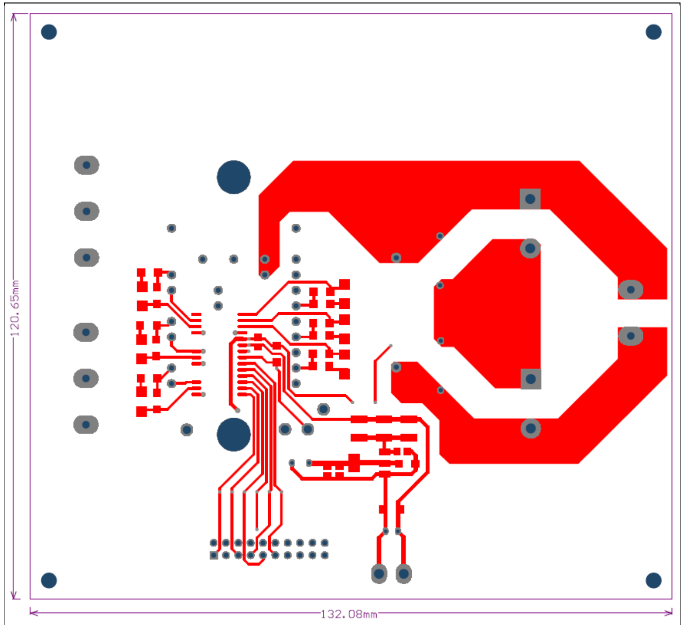
Figure 11 Top layer routing of the EVAL-M1-6ED2230-B1 evaluation board
