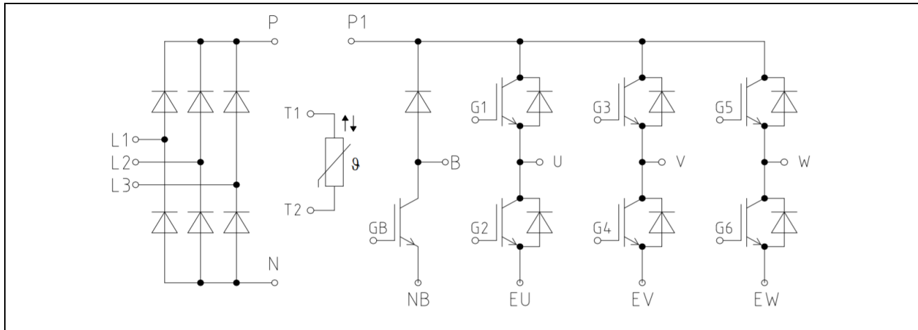
Figure 6 Schematic of the 3-phase inverter section using EasyPIM™ modules FP15R12W1T4 on the EVAL-M1-6ED2230-B1 evaluation board
