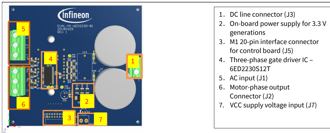
Figure 3 Functional groups of the EVAL-M1-6ED2230-B1 evaluation board's top side
