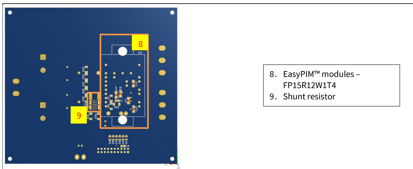
Figure 4 Functional groups of the EVAL-M1-6ED2230-B1 evaluation board's bottom side (heatsink is removed)
