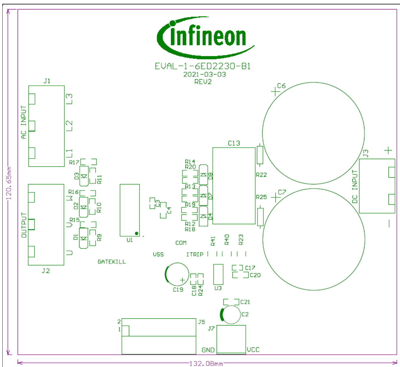
Figure 9 Top assembly print of the EVAL-M1-6ED2230-B1 evaluation board
