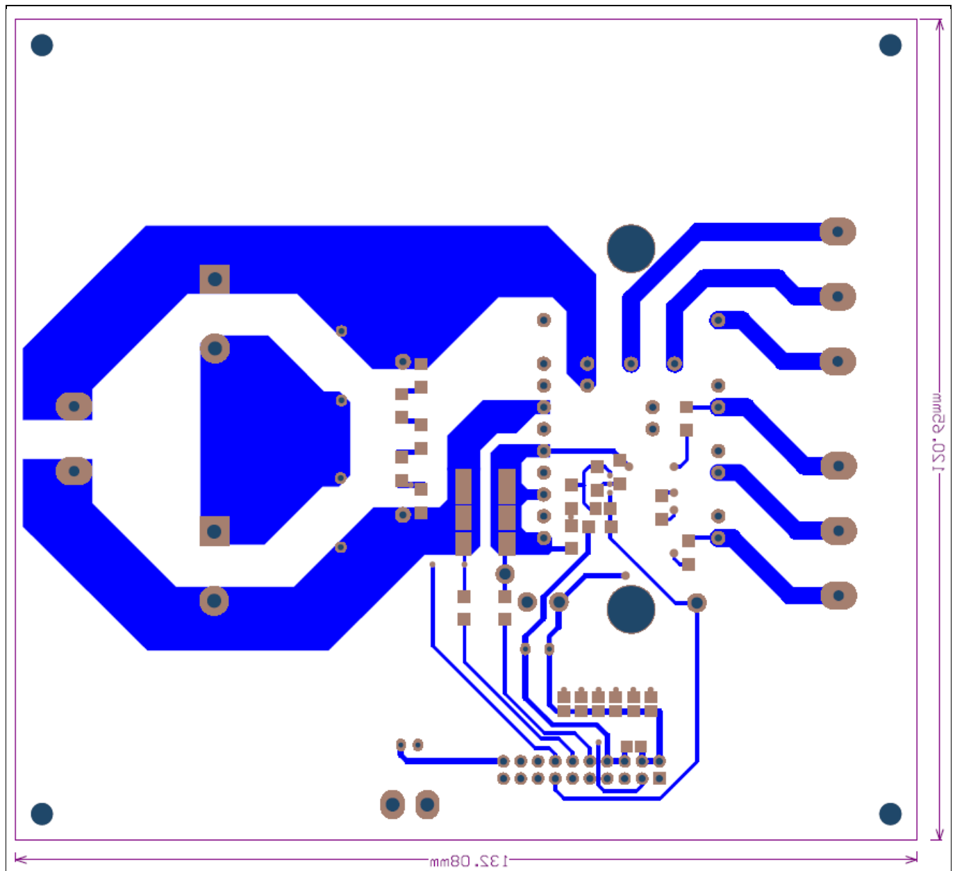
Figure 12 Bottom layer routing of the EVAL-M1-6ED2230-B1 evaluation board
