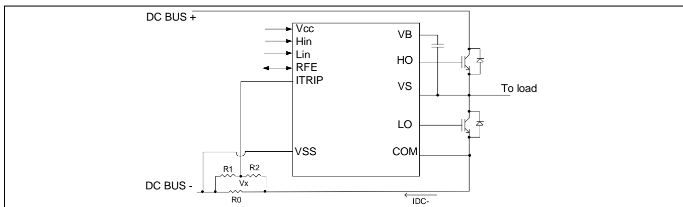
Figure 2 Typical connection of the 6ED2230S12T gate driver IC
