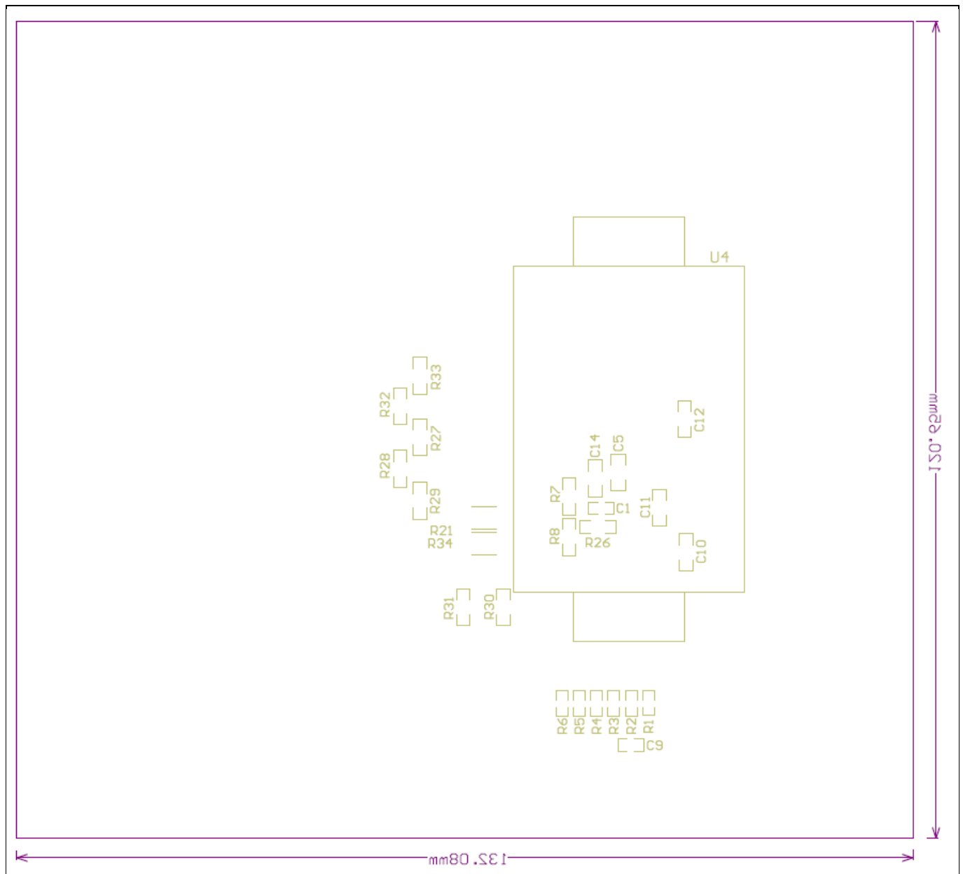
Figure 10 Bottom assembly print of the EVAL-M1-6ED2230-B1 evaluation board
