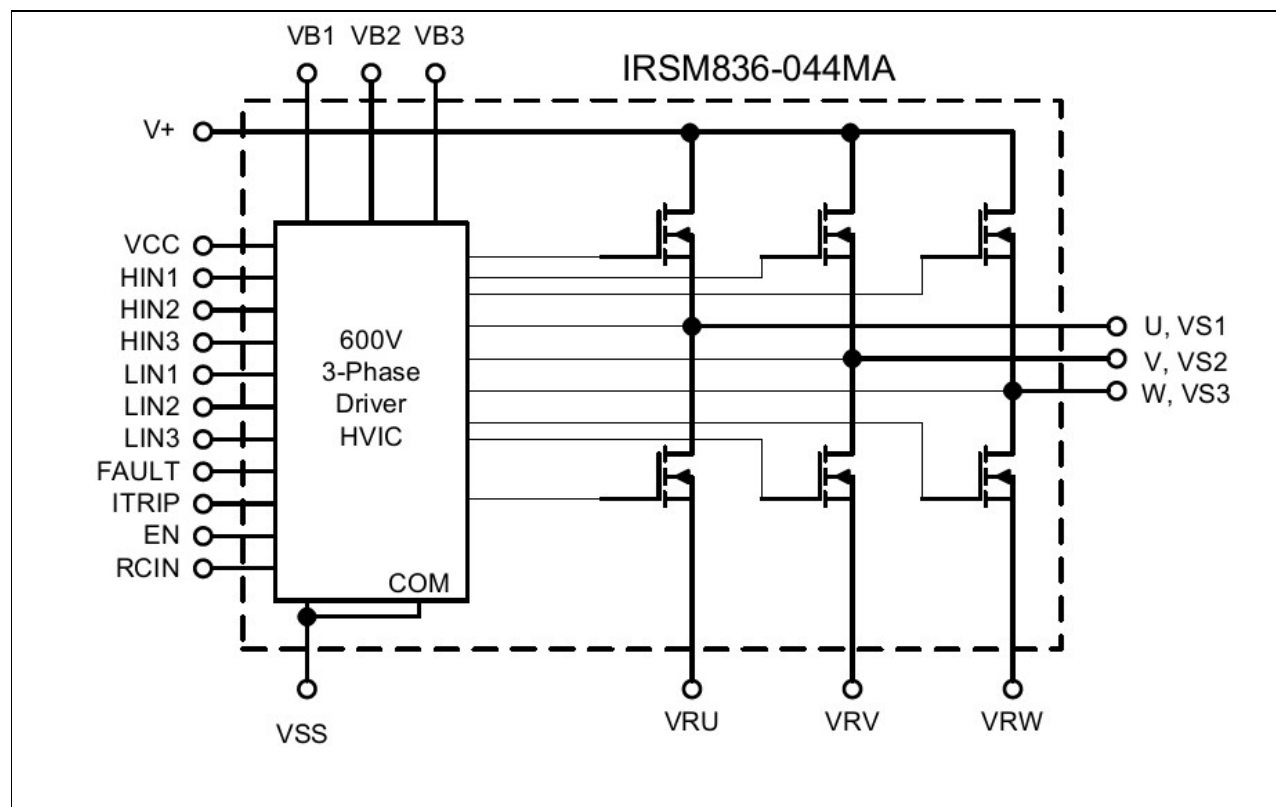
Figure 2 CIPOS™ Nano internal electrical schematic
