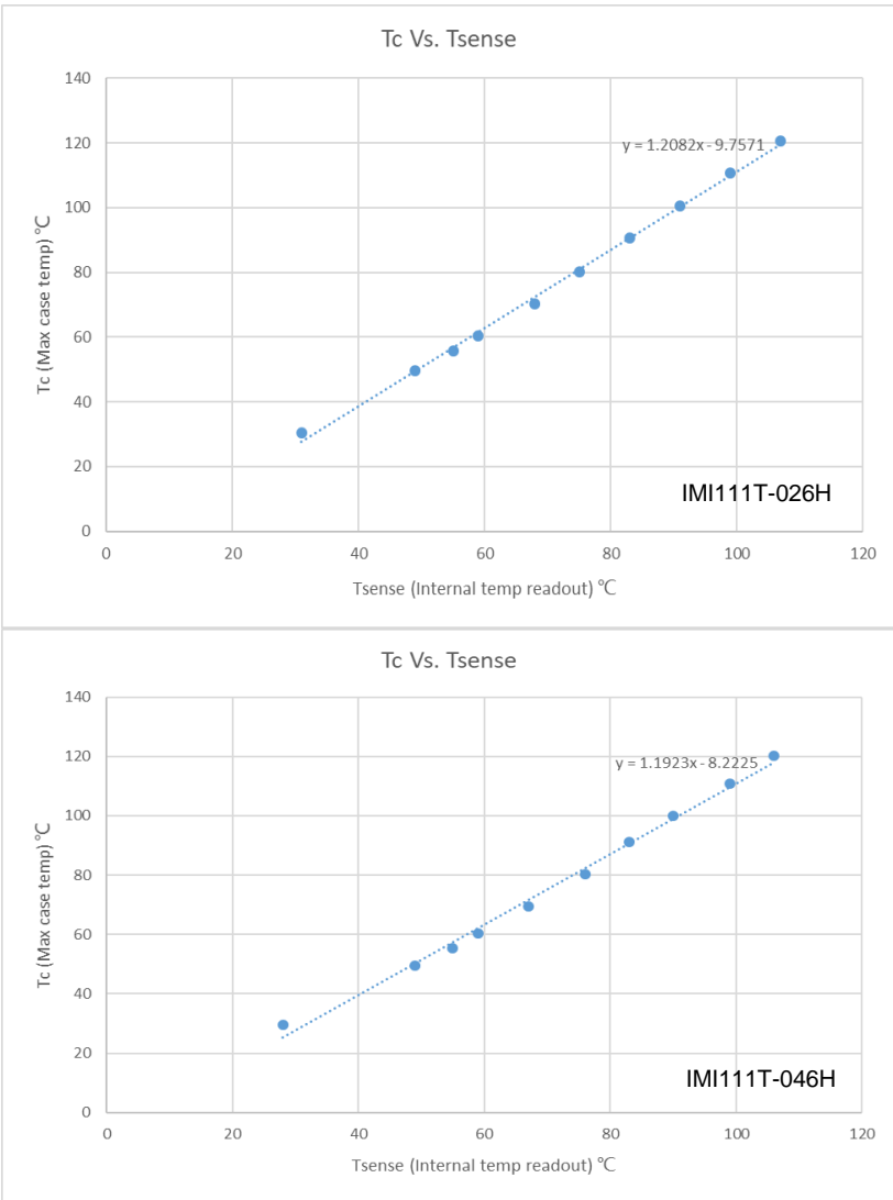
Figure 22 Correlation between the case temperature and the internal temperature readout
