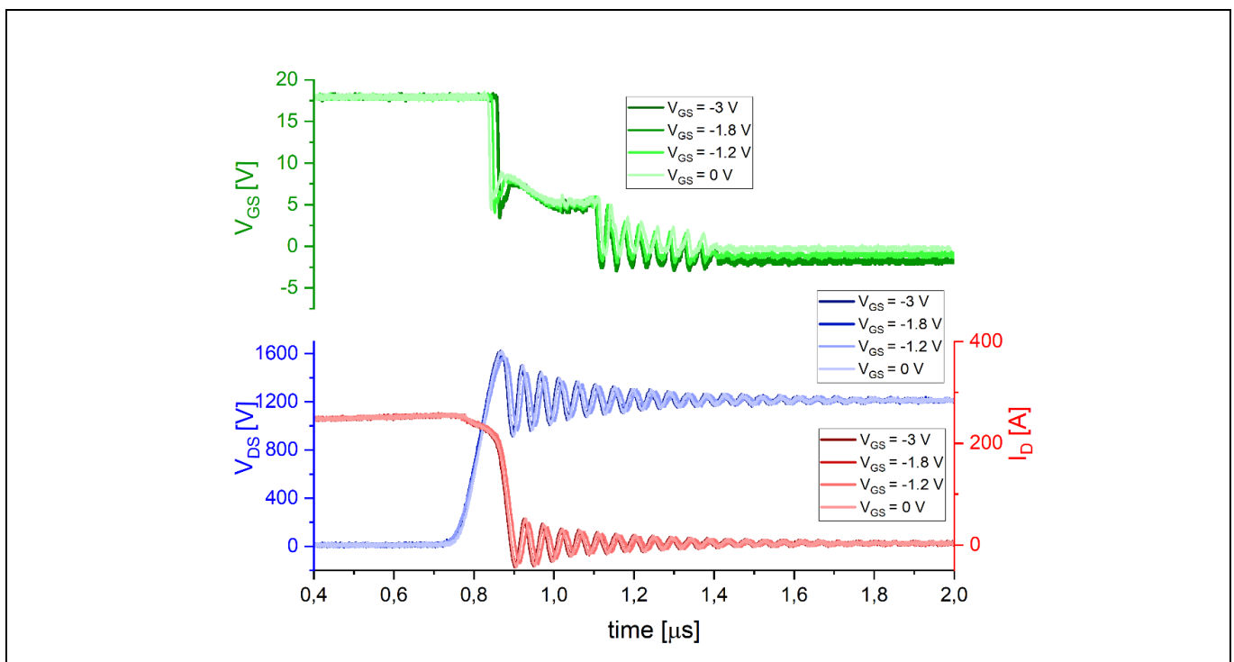
Figure 19 Turn-off waveforms with different ( V_{GS} = -3... 0\text{ V} / +18\text{ V} )
