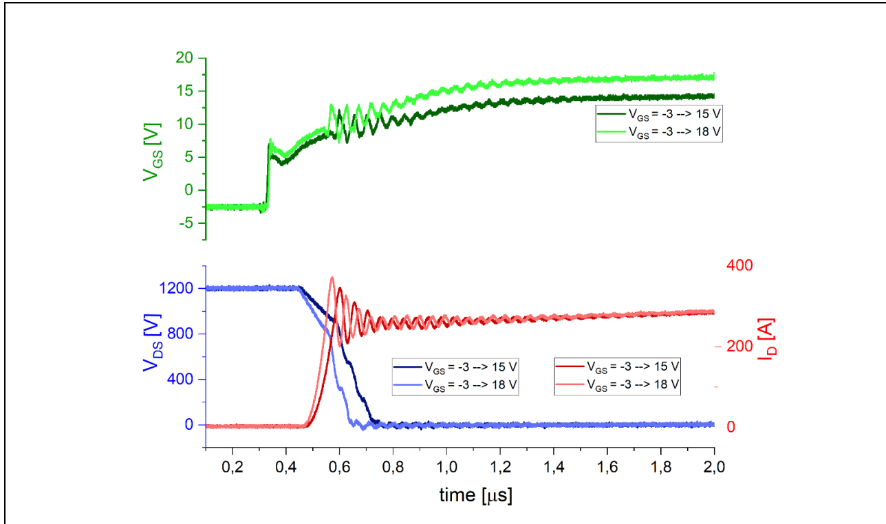
Figure 18 Turn on waveforms of typical bipolar voltage values with V_{GS} = -3...+15\text{ V} / ...+18\text{ V} .
