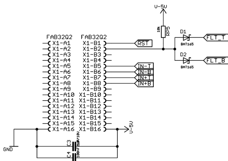
Figure 4-3 connector X1
