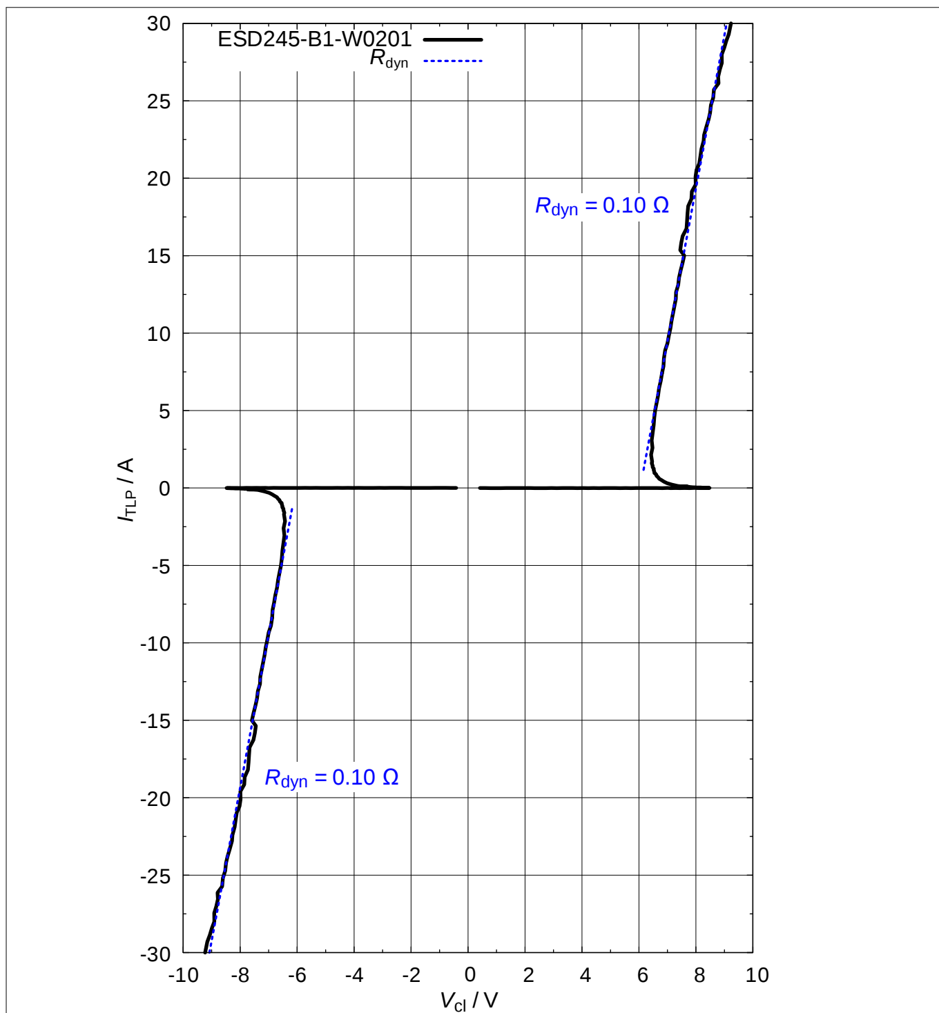
Figure 9 Clamping voltage (TLP): I_{TLP} = f(V_{TLP})
