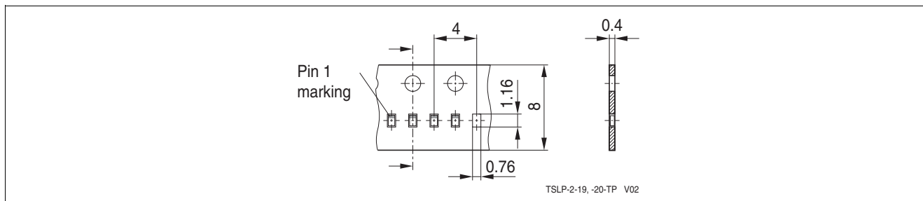
Figure 4-3 TSLP-2-19 Packing
