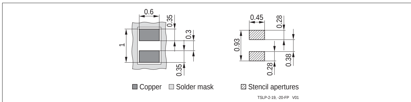
Figure 4-2 TSLP-2-19 Footprint
