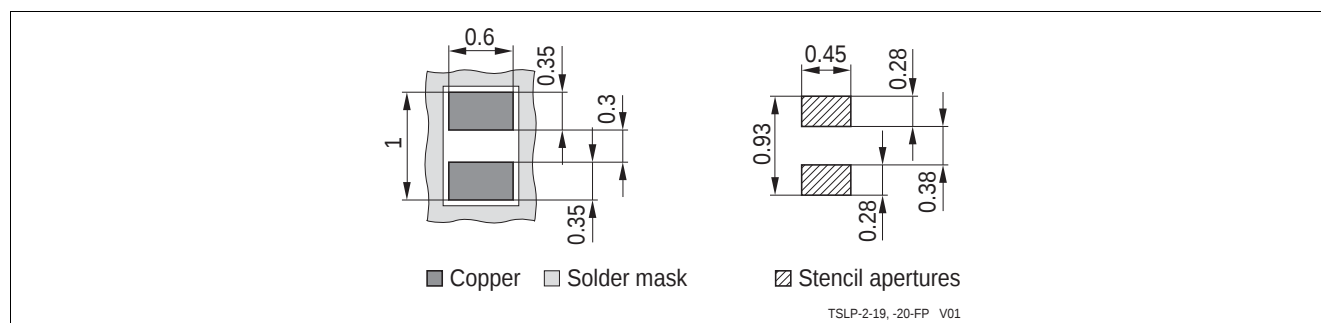
Figure 5-6 TSLP-2-19 Footprint
