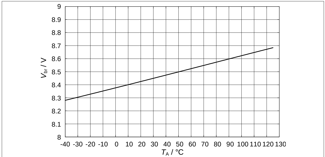
Figure 5 Breakdown voltage V_{br} = f(T_A) , I_t = 1 mA
