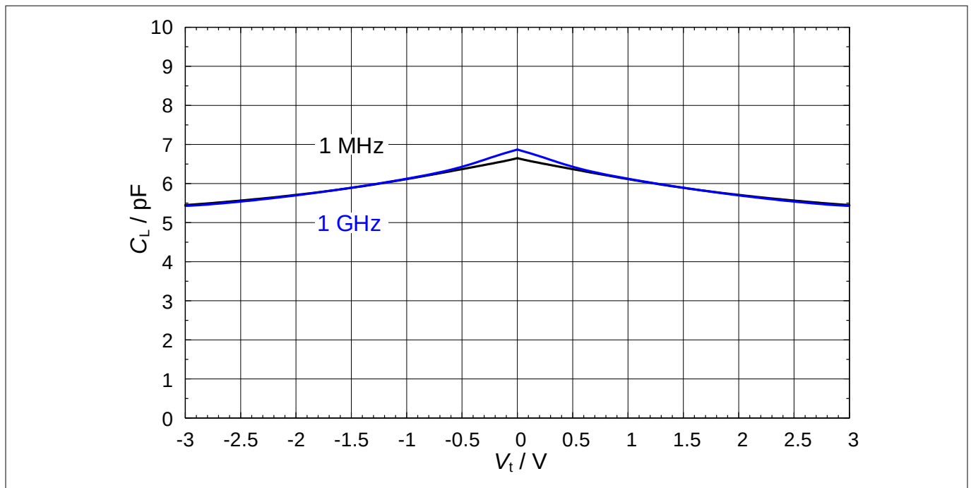
Figure 6 Line capacitance: C_L = f(V_t) , f = 1 MHz, 1 GHz
