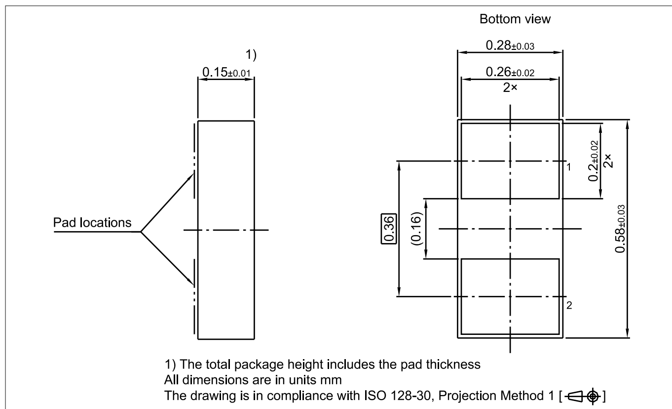
Figure 14 WLL-2-1 package
