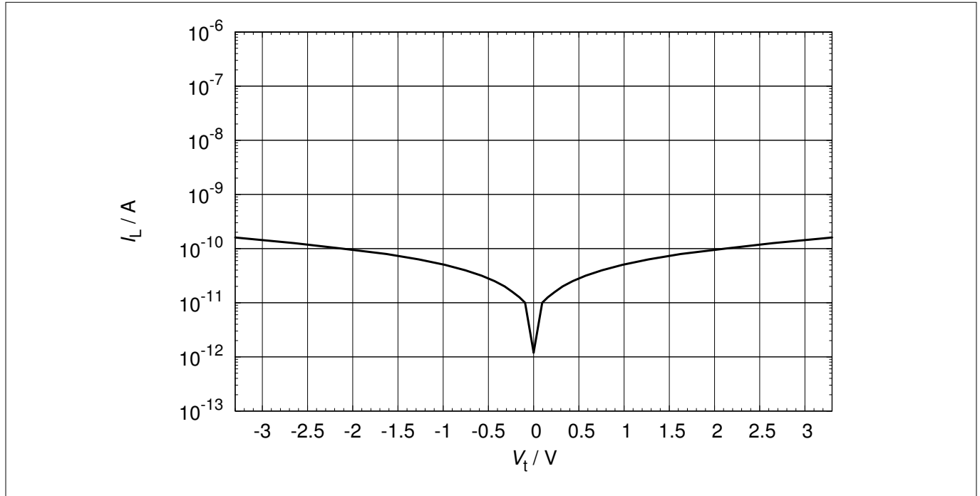
Figure 3 Leakage current: I_L = f(V_t)
