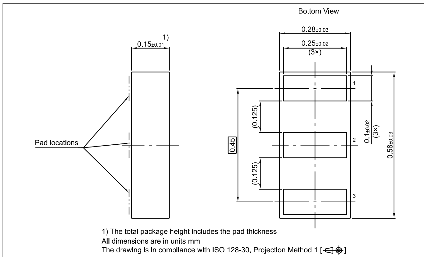
Figure 13 WLL-3-1 package
