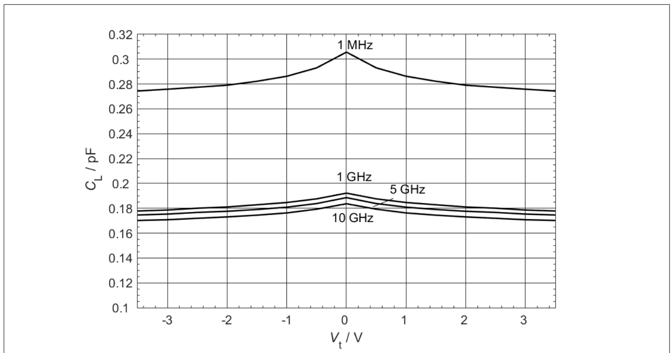
Figure 4 Line capacitance: C_L = f(V_t) , f = 1\text{ MHz}, 1\text{ GHz}, 5\text{ GHz}, 10\text{ GHz}
