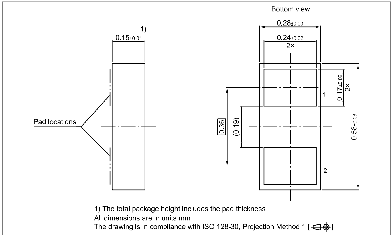
Figure 15 WLL-2-3 package
