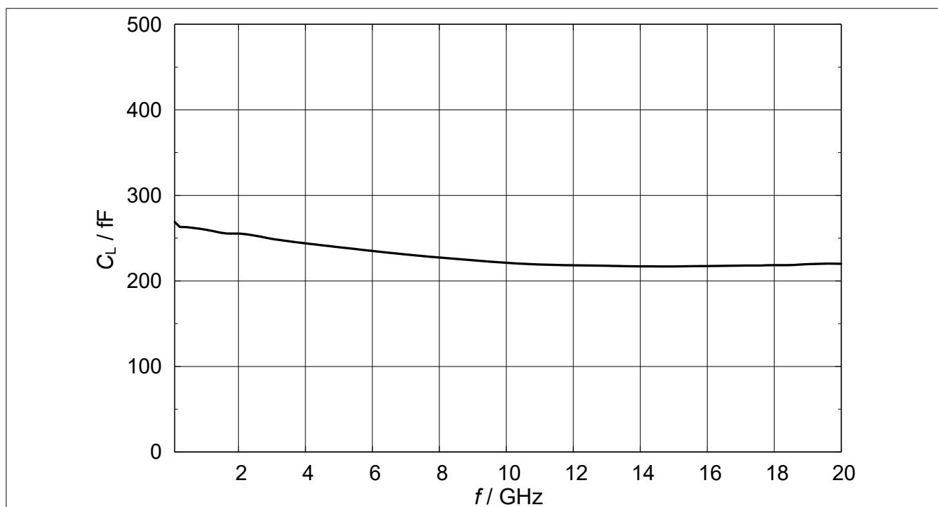
Figure 5 Line capacitance: C_L = f(f) = 1 MHz
