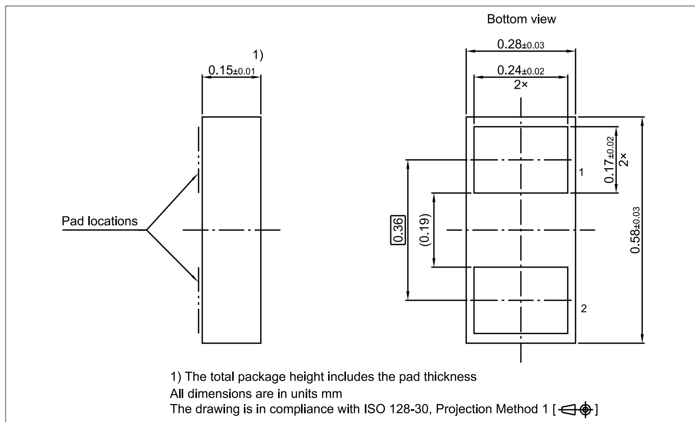
Figure 15 WLL-2-3 package
