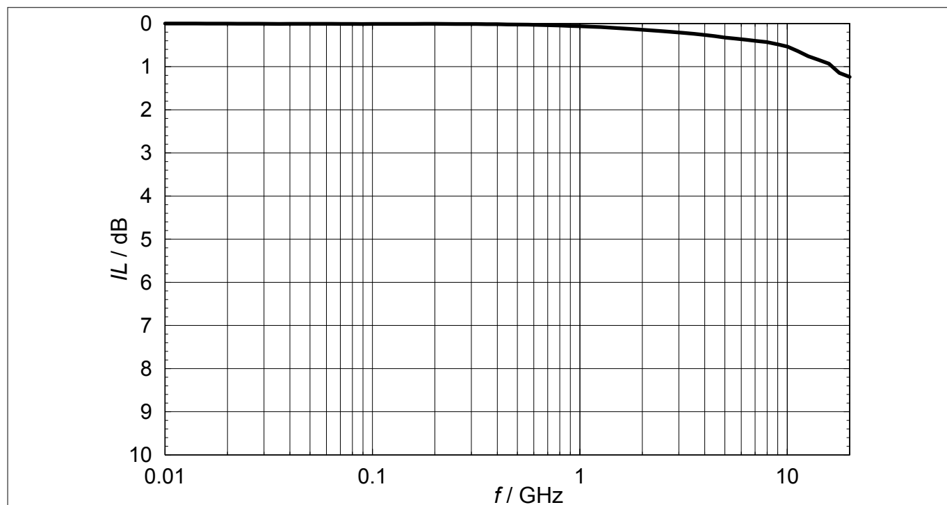
Figure 11 Insertion loss IL = f(f) , measured in a 50 \Omega system
