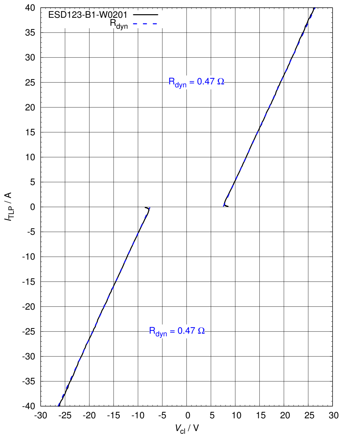
Figure 9 Clamping voltage (TLP): I_{TLP} = f(V_{cl})
