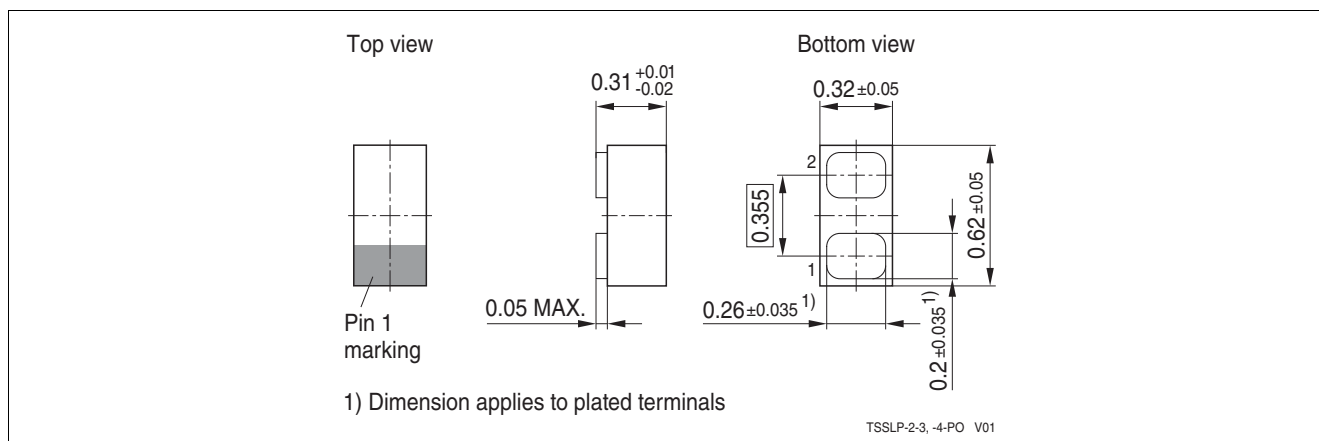
Figure 10 TSSLP-2-3: Package overview
