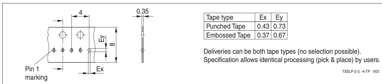
Figure 12 TSSLP-2-3: Packing
