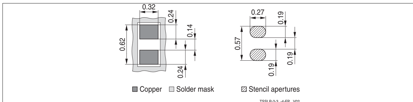
Figure 11 TSSLP-2-3 Footprint
