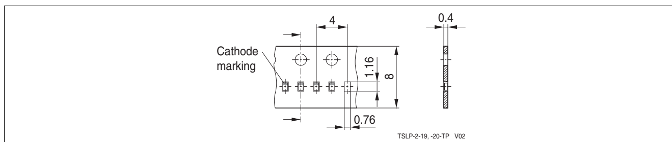
Figure 4-7 TSLP-2-20: Packing
