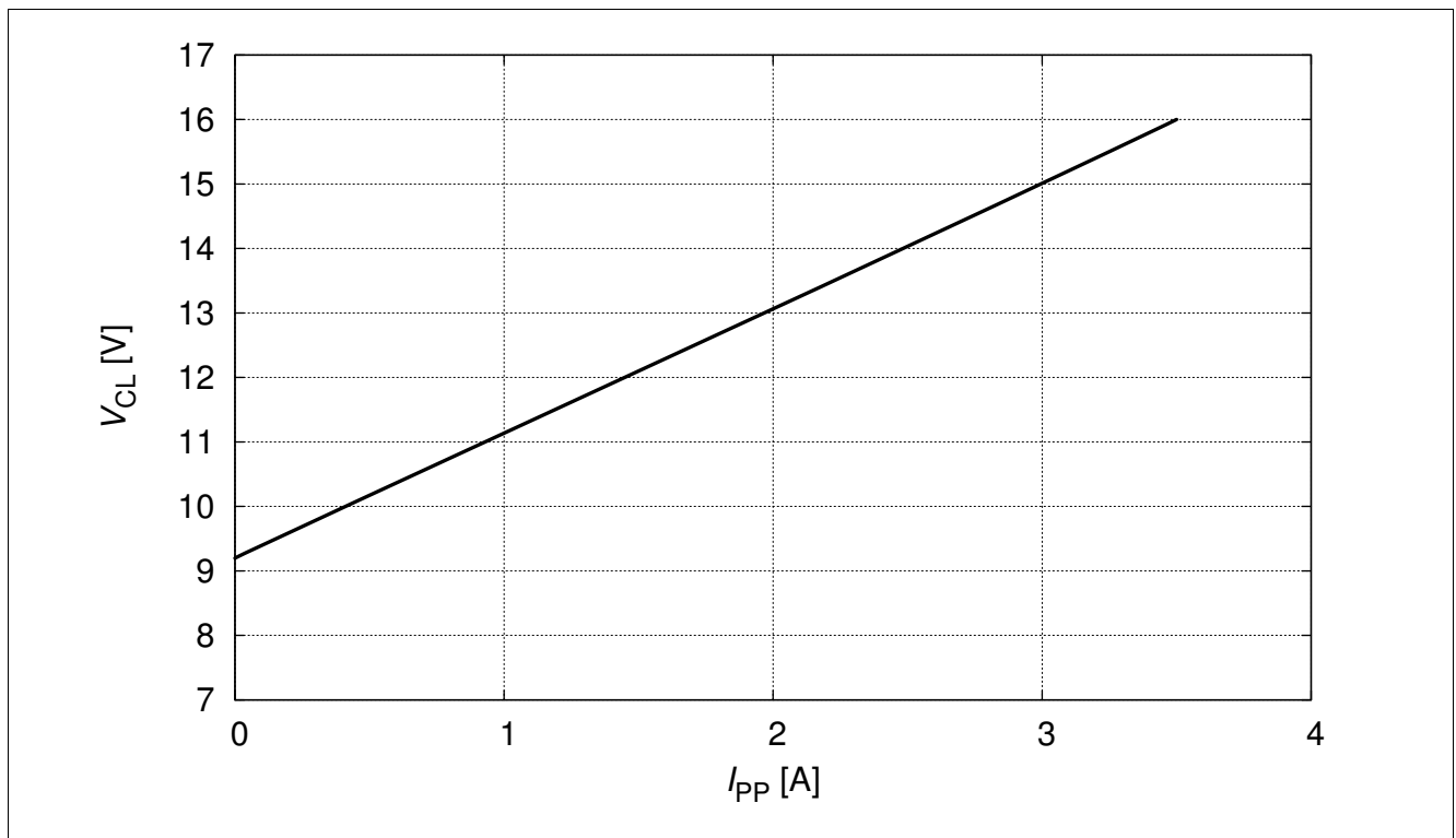
Figure 2-11 Clampine voltage: V_{CL} = f(I_{PP}) , t_p = 8/20 \mu s
