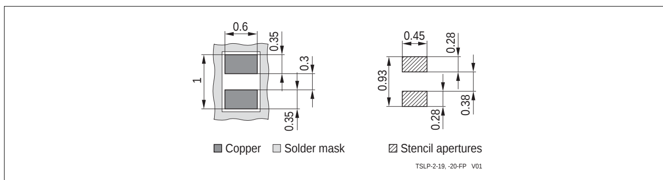
Figure 4-6 TSLP-2-20: Footprint
