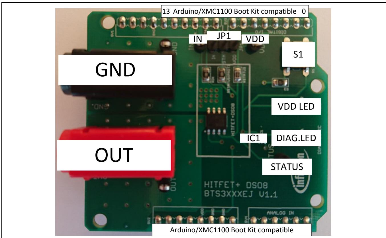
Figure 1 Board Overview
