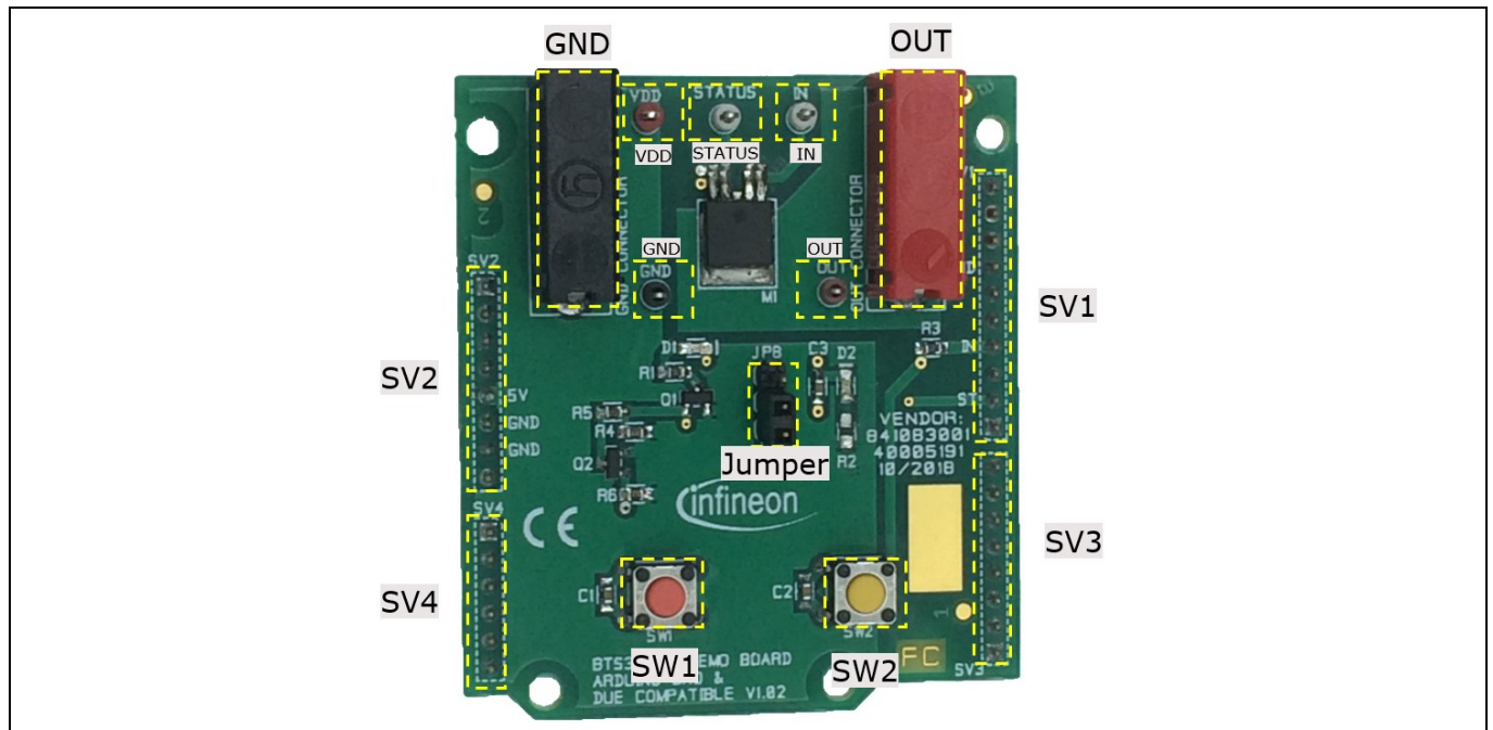
Figure 10 Connectors implantation
