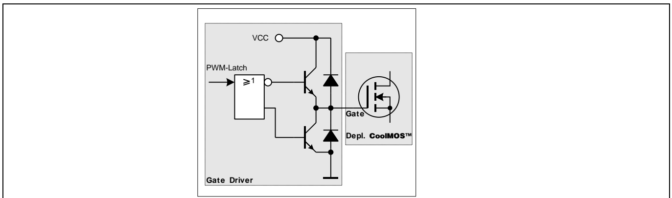
Figure 8 Gate Driver
