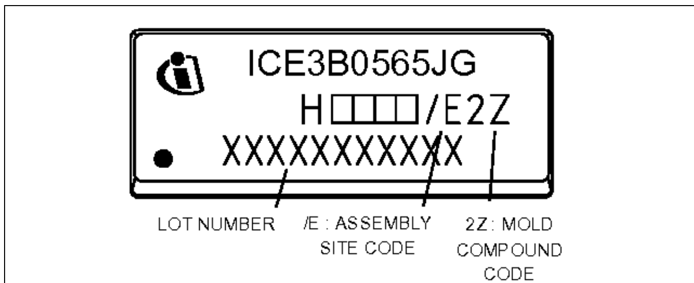
Figure 21 Marking for ICE3B0565JG
