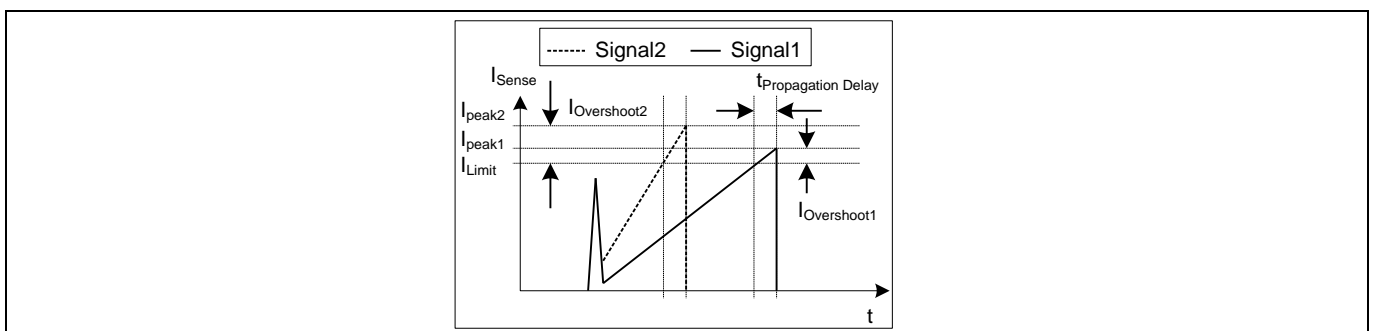
Figure 11 Current Limiting
