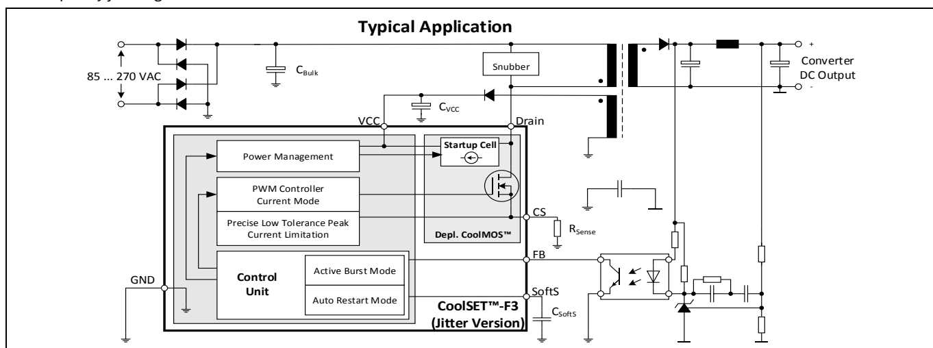
Figure 1 Typical application
