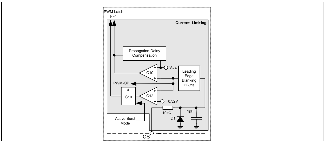
Figure 9 Current Limiting
