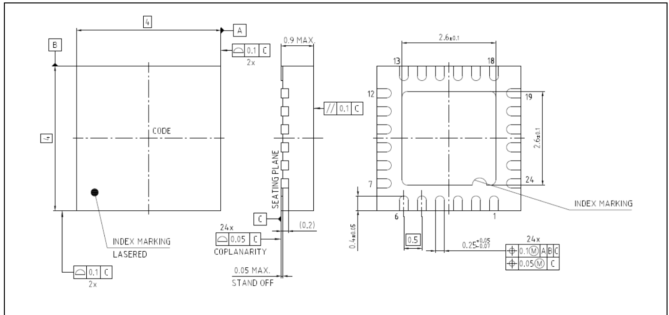
Figure 33 PG-VQFN-24-20
