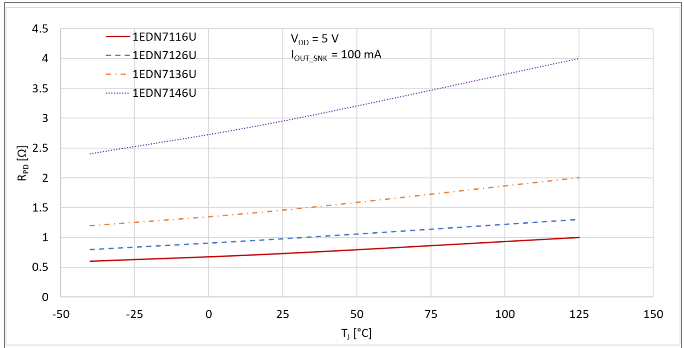
Figure 17 OUT_SNK pull-down resistance versus temperature (before active Miller clamp is engaged)
