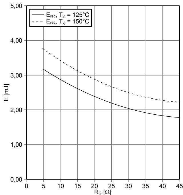
スイッチング損失 Diode-、チョッパ (Typical) switching losses Diode-Chopper (typical) E_{rec} = f(R_G)
