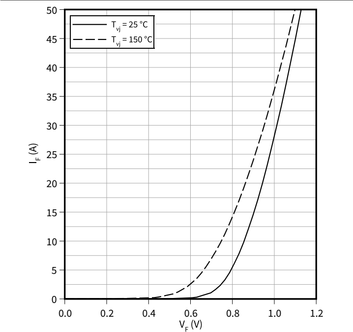
Forward characteristic (typical), Inverse-polarity protection diode B I_F = f(V_F)
