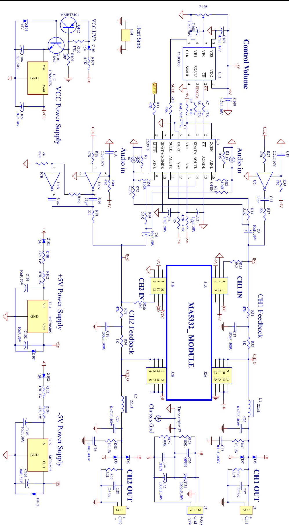
Figure 18 Motherboard schematic 3
