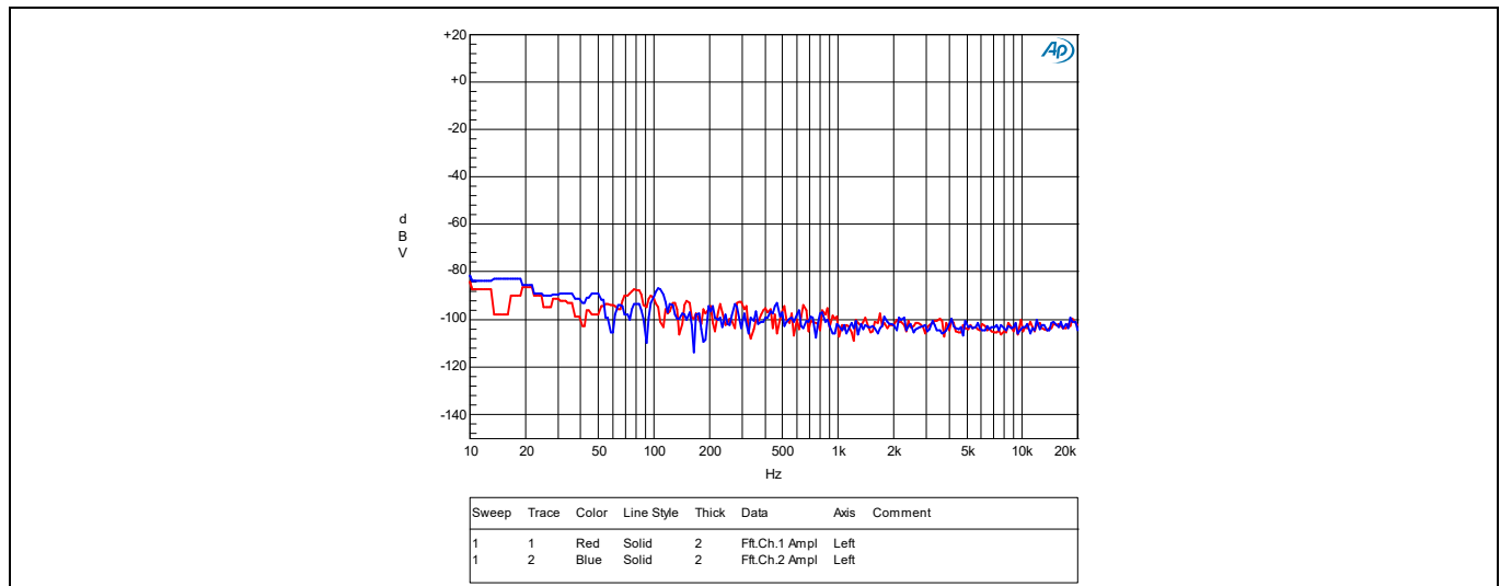
Figure 6 Noise floor 4 \Omega load
