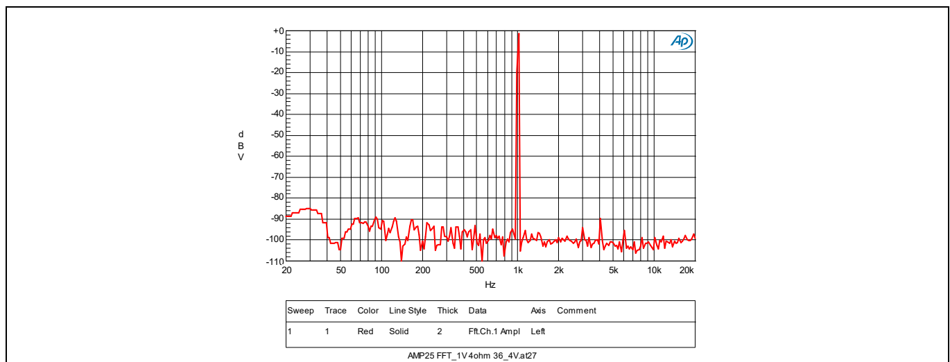
Figure 7 Noise floor with 1 V_{\text{RMS}} output 4 \Omega load
