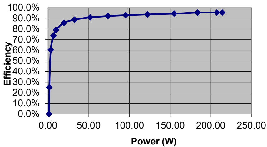
Figure 8 EVAL_AUDAMP25 4 \Omega load stereo, \pm B supply = \pm 36.5 \text{ V}
