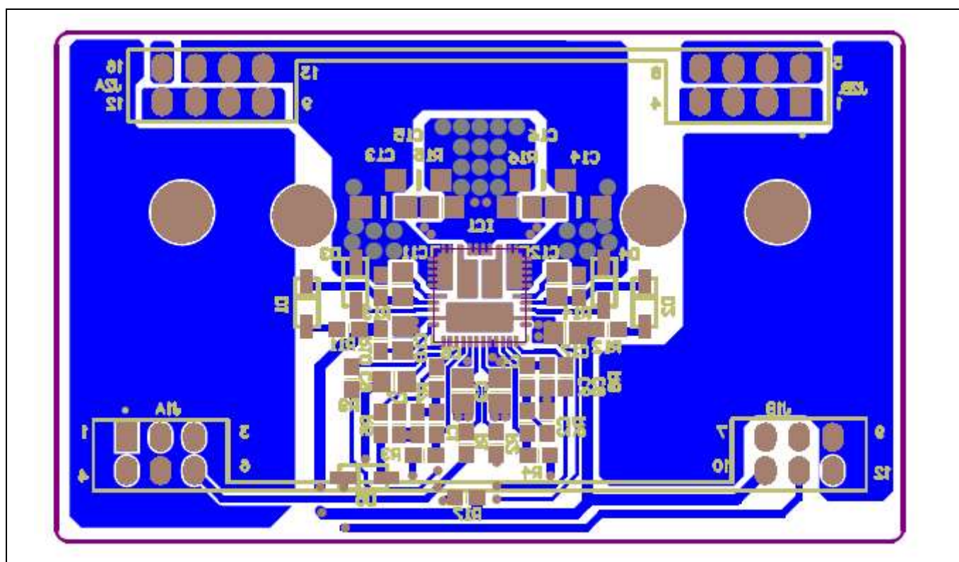
Figure 23 Daughterboard bottom view
