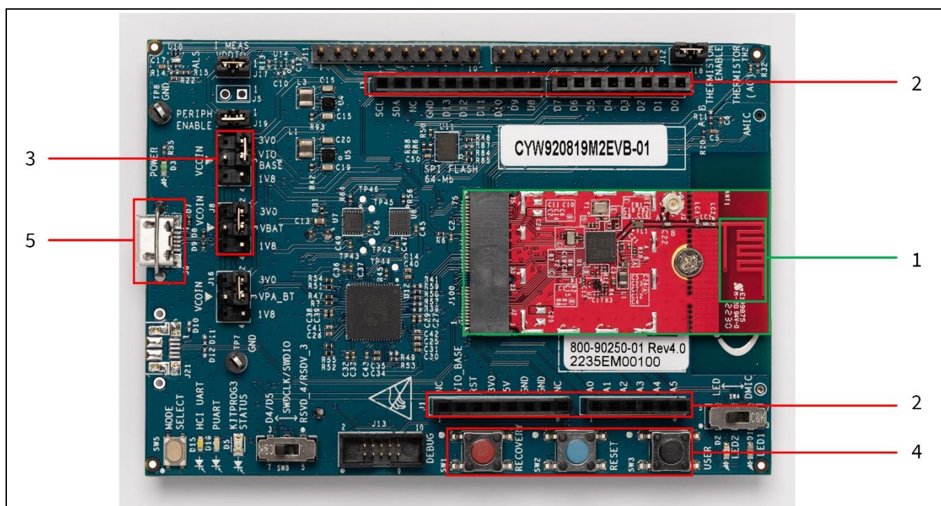
Figure 2 CYW920819M2EVB-01 evaluation board
