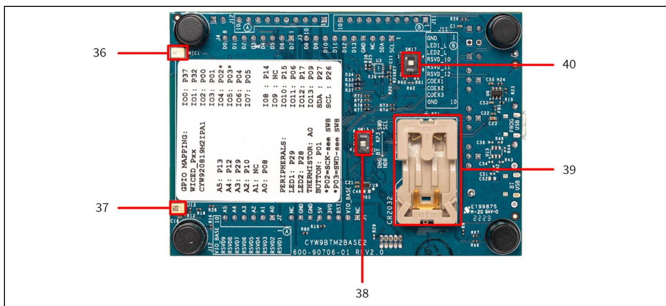
Figure 9 CYW920819M2EVB-01 evaluation board (Bottom view)
