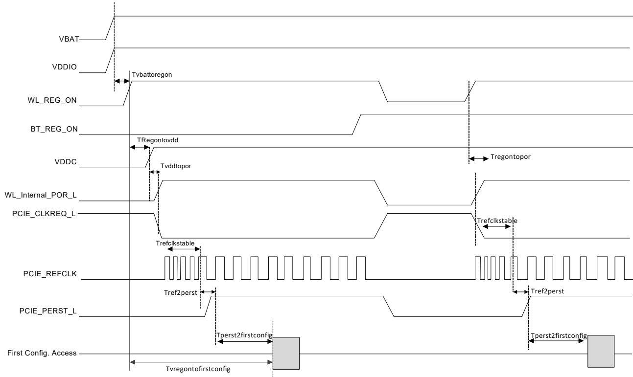
Figure 48. WLAN/PCle Power-Up Timing
