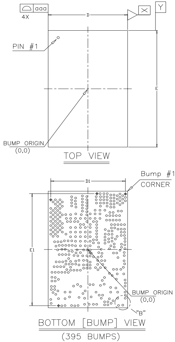
Figure 51. 395-Bump WLCSP Package
