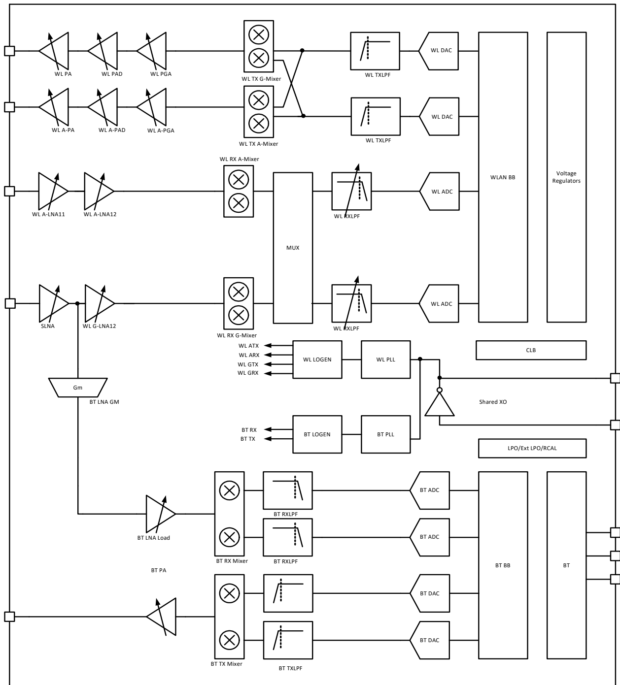
Figure 30. Radio Functional Block Diagram (Core 0)
