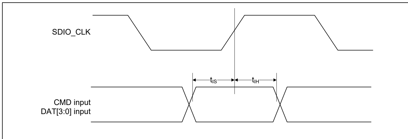
Figure 34. SDIO Bus Input Timing (SDR Modes)
