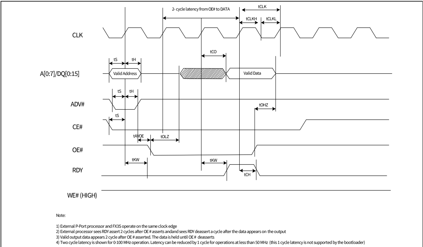
Figure 20 Synchronous ADMux interface – Read cycle timing
