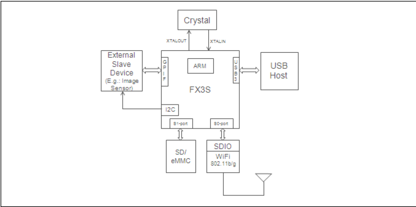
Figure 2 EZ-USB™ FX3S as main processor
