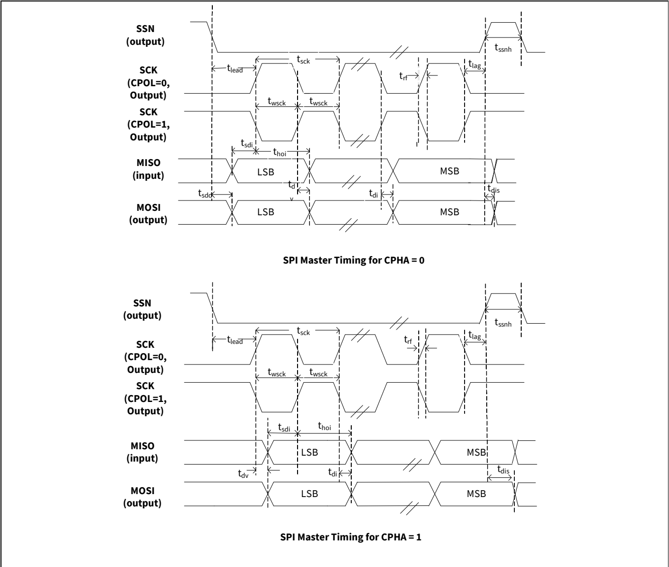
Figure 30 SPI timing
