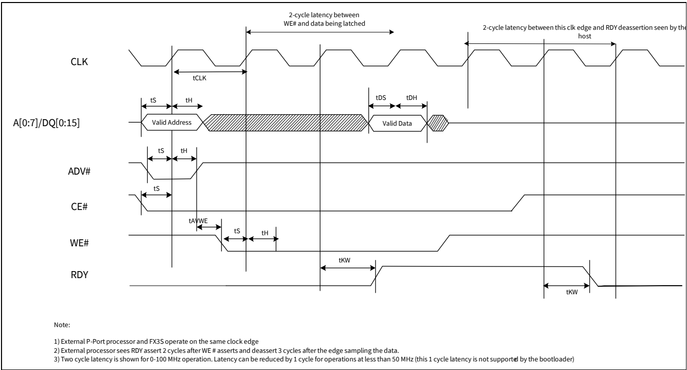
Figure 21 Synchronous ADMux interface – Write cycle timing
