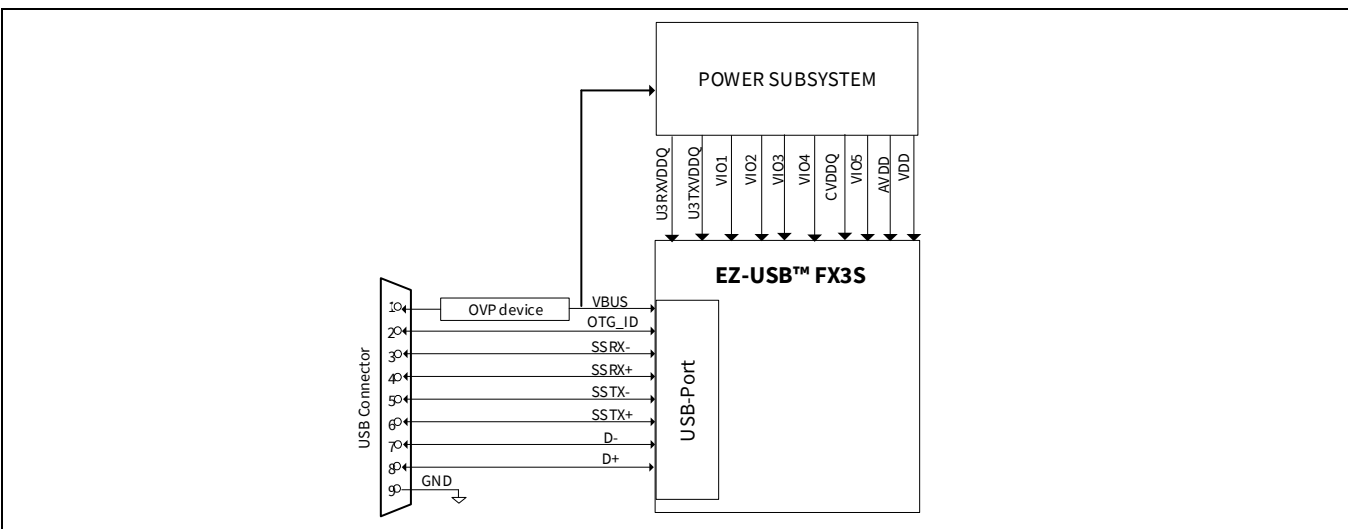
Figure 4 System diagram with OVP device for VBUS
