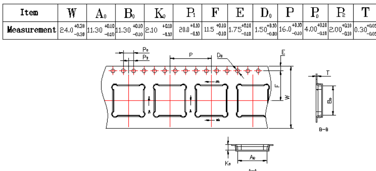
Figure 20. CYBT-4230xx-02 Tape Dimensions
