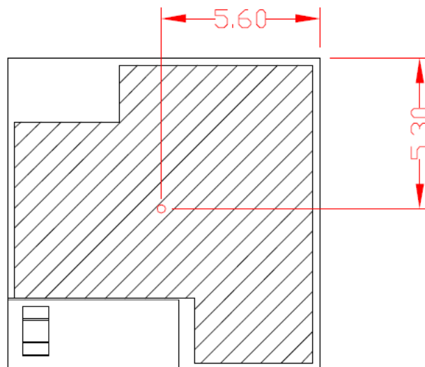
Figure 23. CYBT-4230xx-02 Center of Mass
