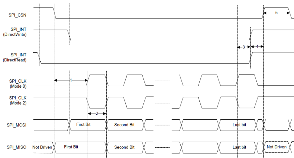
Figure 15. SPI Timing, Mode 0 and 2
