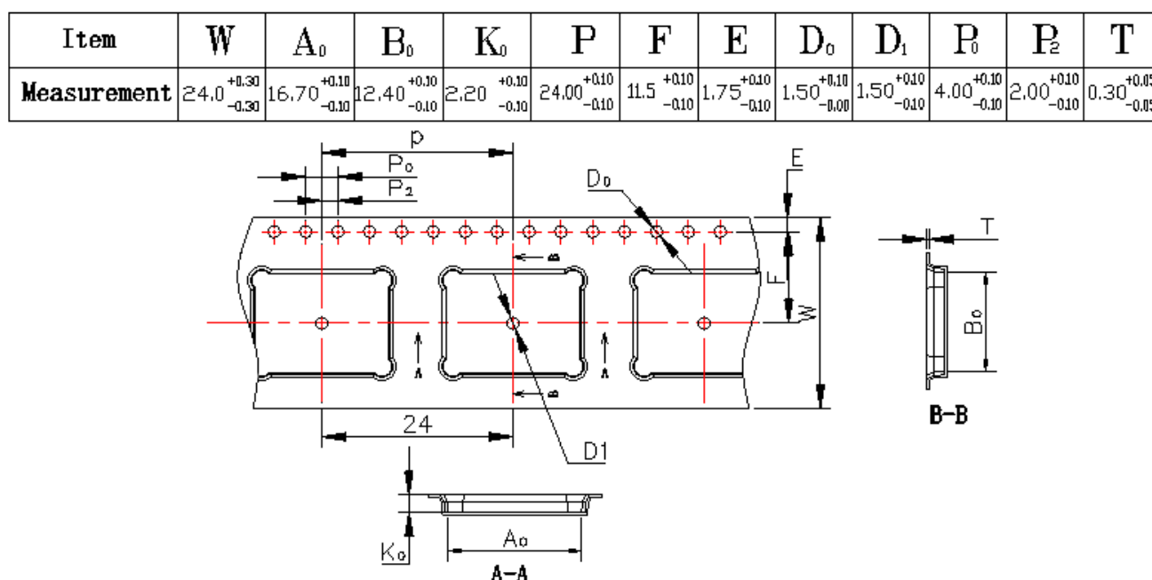
Figure 20. CYBT-4130xx-02 Tape Dimensions
