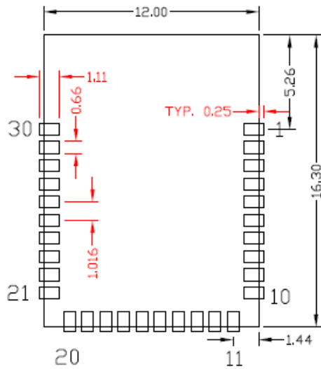
Figure 5. CYBT-4130xx-02 Host Layout (Dimensioned)
