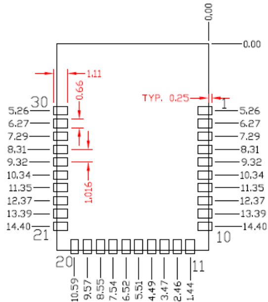
Figure 6. CYBT-4130xx-02 Host Layout (Relative to Origin)
