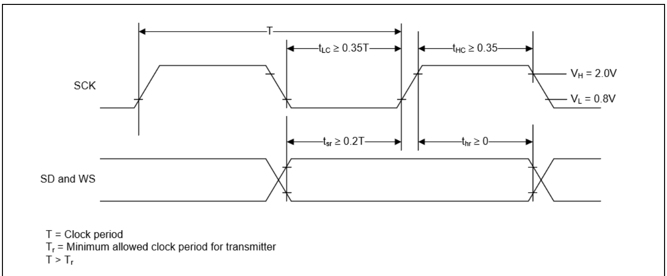
Figure 18 I²S Receiver Timing
