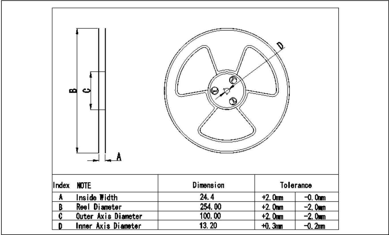
Figure 21 Reel dimensions
