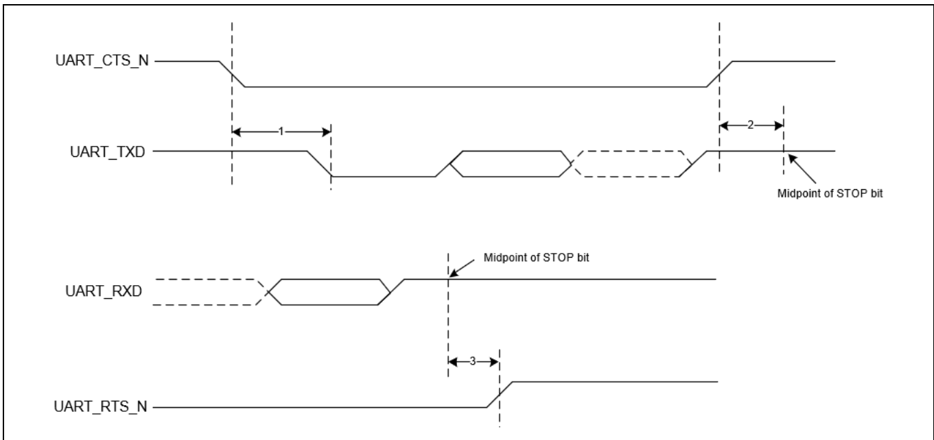
Figure 13 UART Timing
