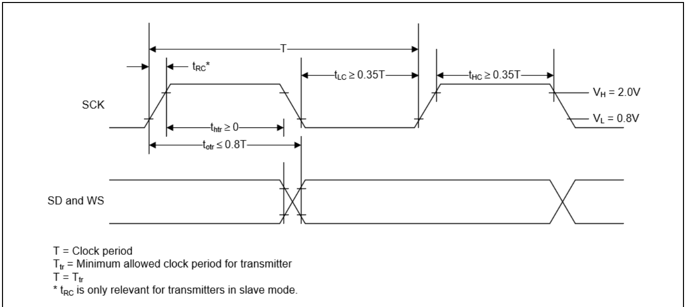
Figure 17 I²S Transmitter Timing
