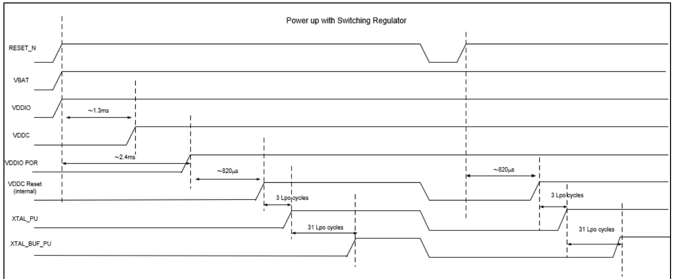
Figure 10 Reset Timing
