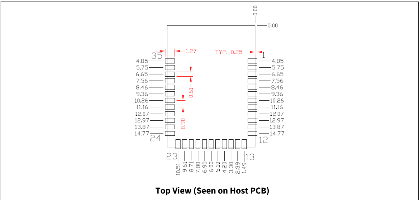
Figure 6 CYBT-243053-02 Host layout (Relative to Origin)
