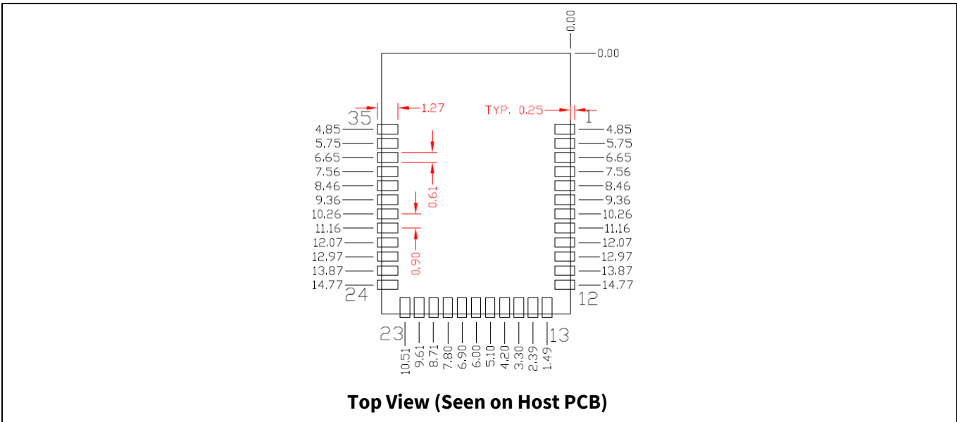
Figure 6 CYBT-213043-02 Host layout (Relative to Origin)
