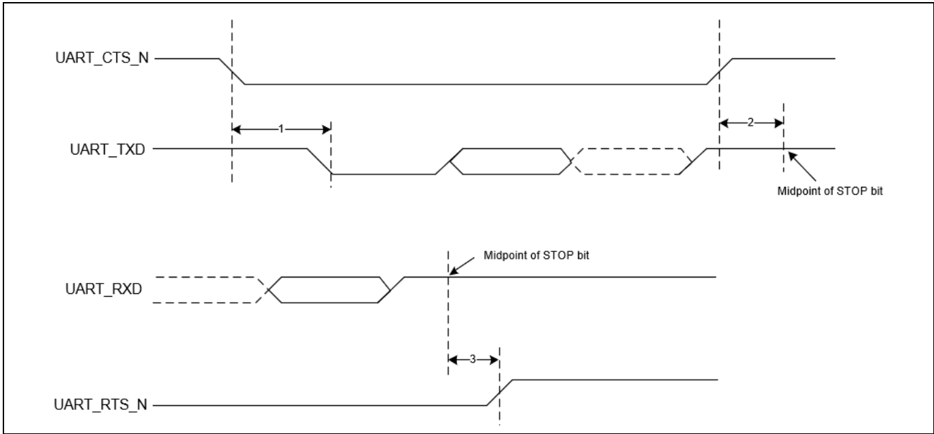
Figure 13 UART Timing
