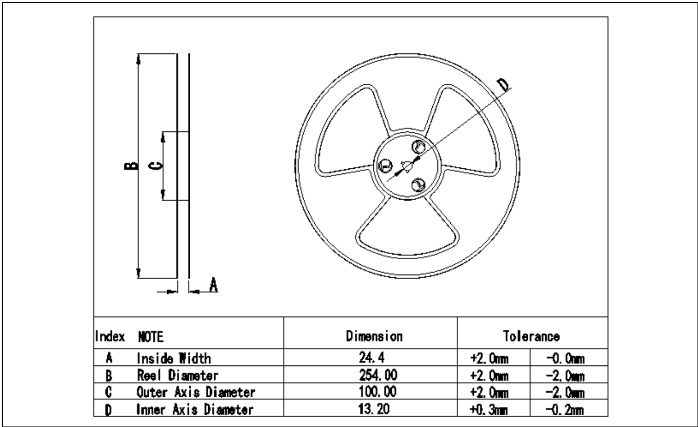
Figure 21 Reel dimensions
